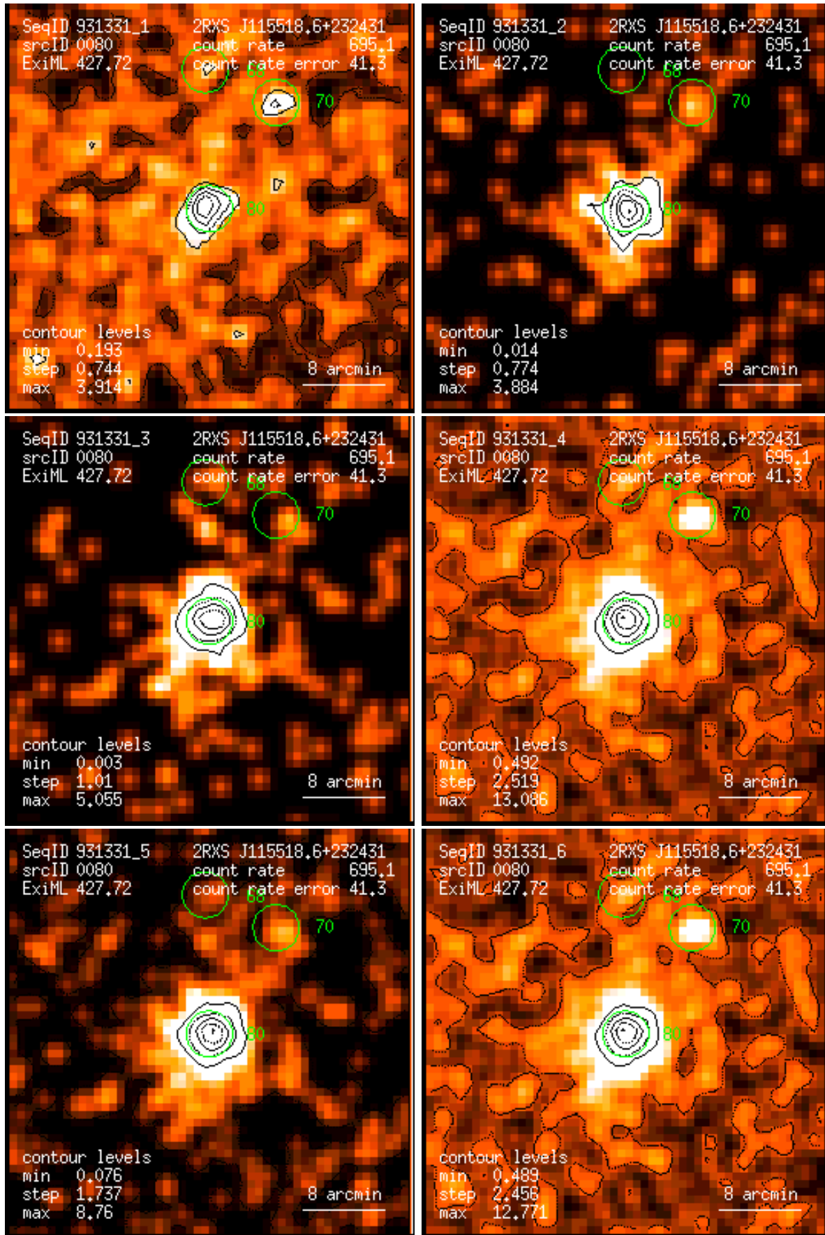
Figure 80: RASS 931331: detection 0080: band rate images, Gaussian filter: (1) PSPC channels 11 – 41, (2) 52 – 90, (3) 91 – 201, (4) 11 – 235, (5) 52 – 201, (6) 11 – 201. Broad band rates in counts/ks. Band rate contour levels in counts/ks/arcmin 2 .
