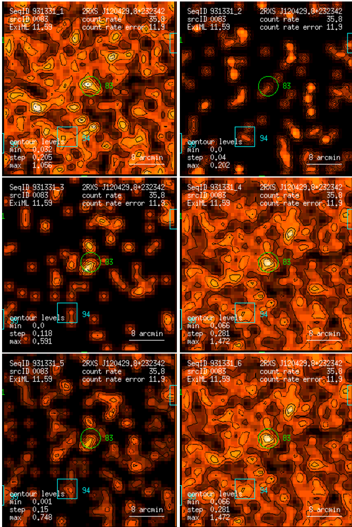
Figure 83: RASS 931331: detection 0083: band rate images, Gaussian filter: (1) PSPC channels 11 – 41, (2) 52 – 90, (3) 91 – 201, (4) 11 – 235, (5) 52 – 201, (6) 11 – 201. Broad band rates in counts/ks. Band rate contour levels in counts/ks/arcmin 2 .
