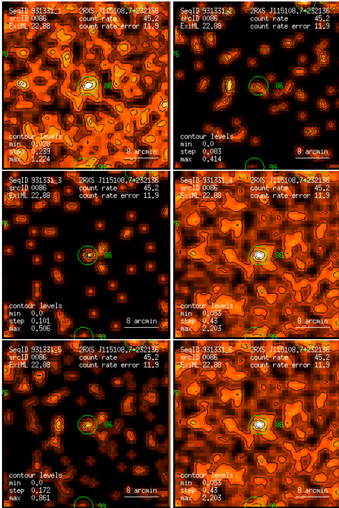
Figure 86: RASS 931331: detection 0086: band rate images, Gaussian filter: (1) PSPC channels 11 – 41, (2) 52 – 90, (3) 91 – 201, (4) 11 – 235, (5) 52 – 201, (6) 11 – 201. Broad band rates in counts/ks. Band rate contour levels in counts/ks/arcmin 2 .
