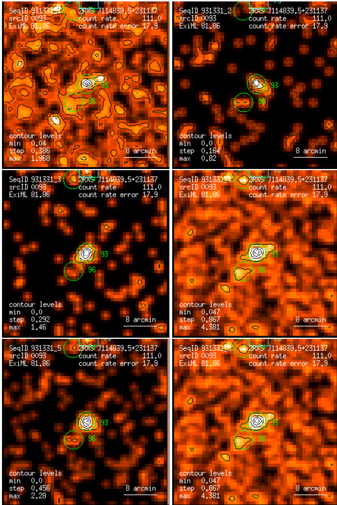
Figure 93: RASS 931331: detection 0093: band rate images, Gaussian filter: (1) PSPC channels 11 – 41, (2) 52 – 90, (3) 91 – 201, (4) 11 – 235, (5) 52 – 201, (6) 11 – 201. Broad band rates in counts/ks. Band rate contour levels in counts/ks/arcmin 2 .
