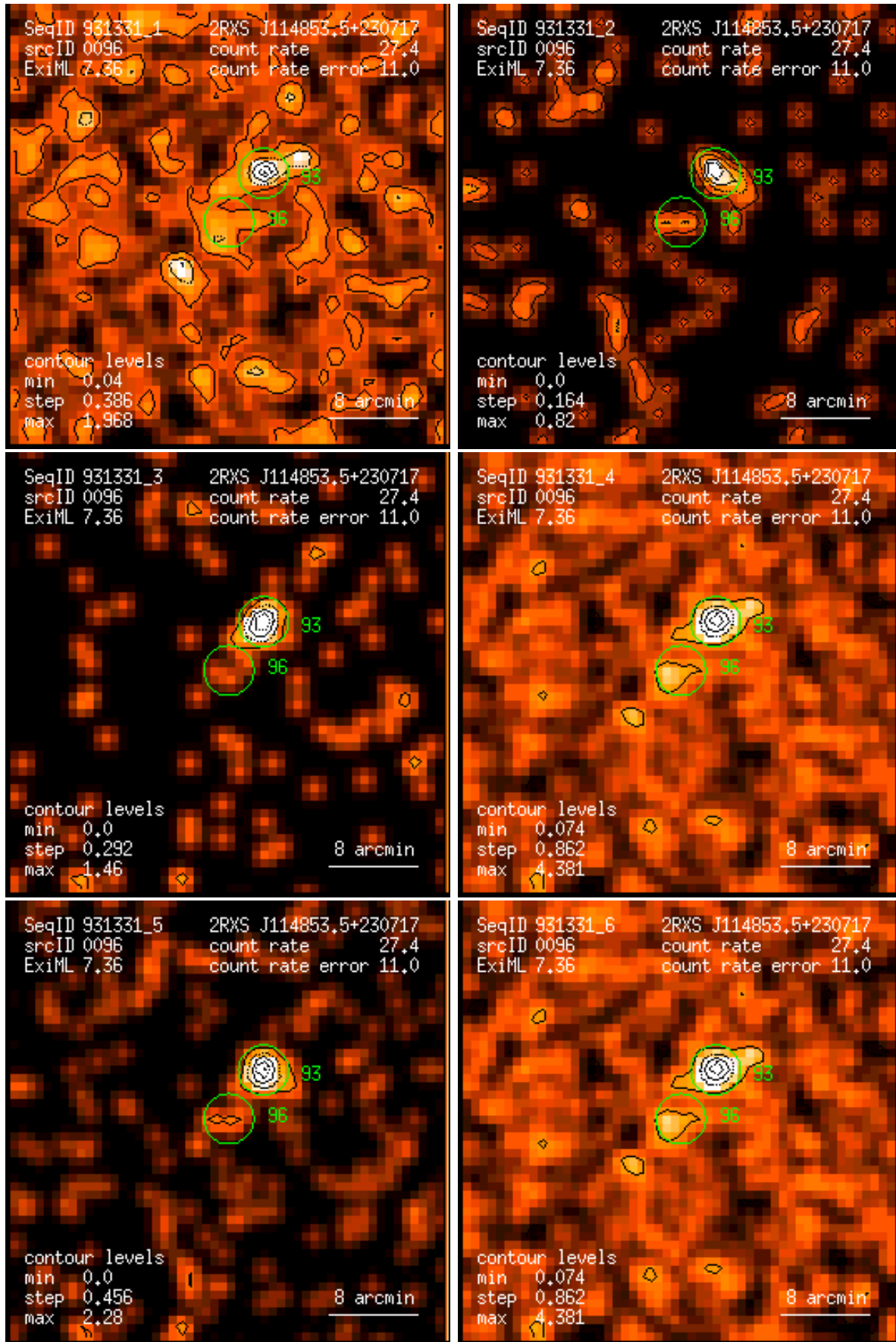
Figure 96: RASS 931331: detection 0096: band rate images, Gaussian filter: (1) PSPC channels 11 – 41, (2) 52 – 90, (3) 91 – 201, (4) 11 – 235, (5) 52 – 201, (6) 11 – 201. Broad band rates in counts/ks. Band rate contour levels in counts/ks/arcmin 2 .
