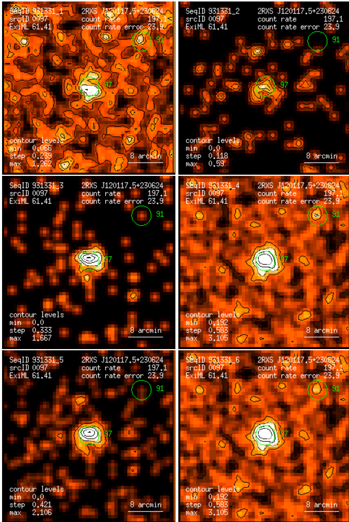
Figure 97: RASS 931331: detection 0097: band rate images, Gaussian filter: (1) PSPC channels 11 – 41, (2) 52 – 90, (3) 91 – 201, (4) 11 – 235, (5) 52 – 201, (6) 11 – 201. Broad band rates in counts/ks. Band rate contour levels in counts/ks/arcmin 2 .
