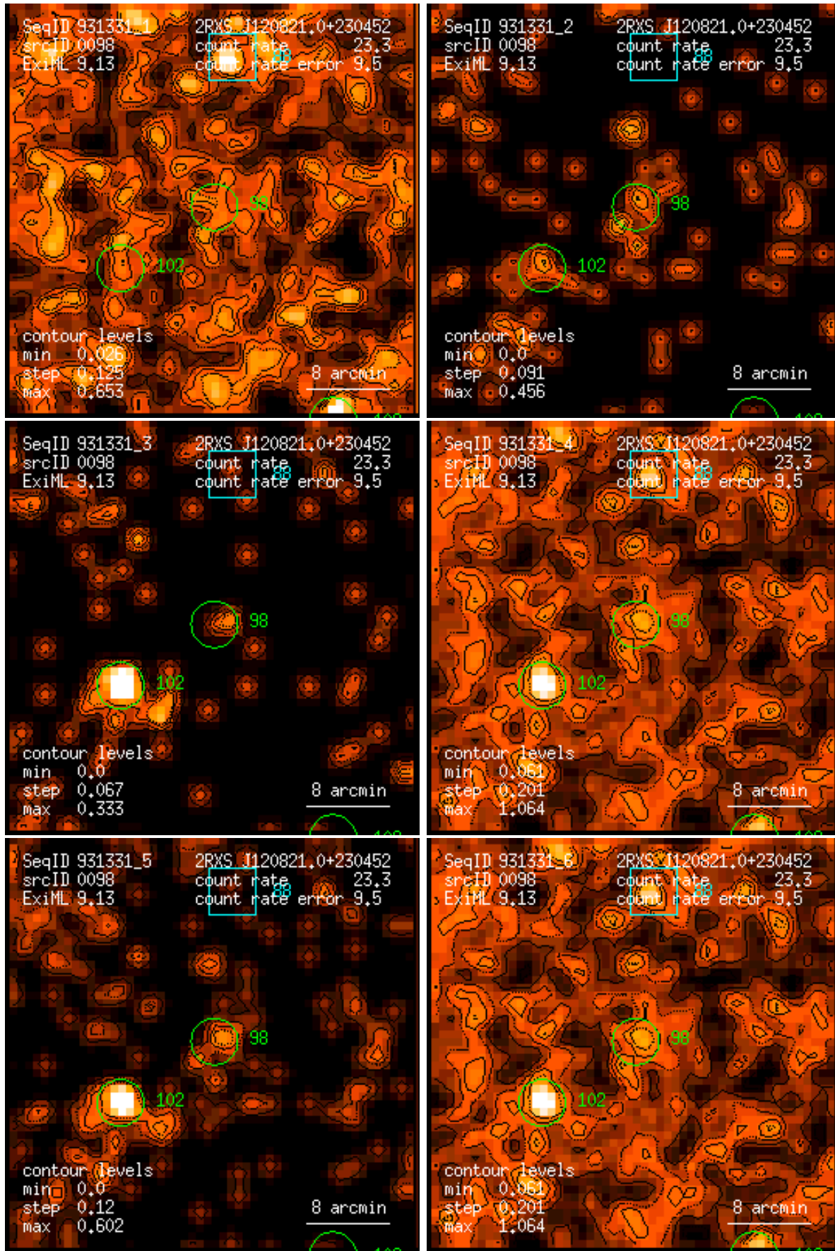
Figure 98: RASS 931331: detection 0098: band rate images, Gaussian filter: (1) PSPC channels 11 – 41, (2) 52 – 90, (3) 91 – 201, (4) 11 – 235, (5) 52 – 201, (6) 11 – 201. Broad band rates in counts/ks. Band rate contour levels in counts/ks/arcmin 2 .
