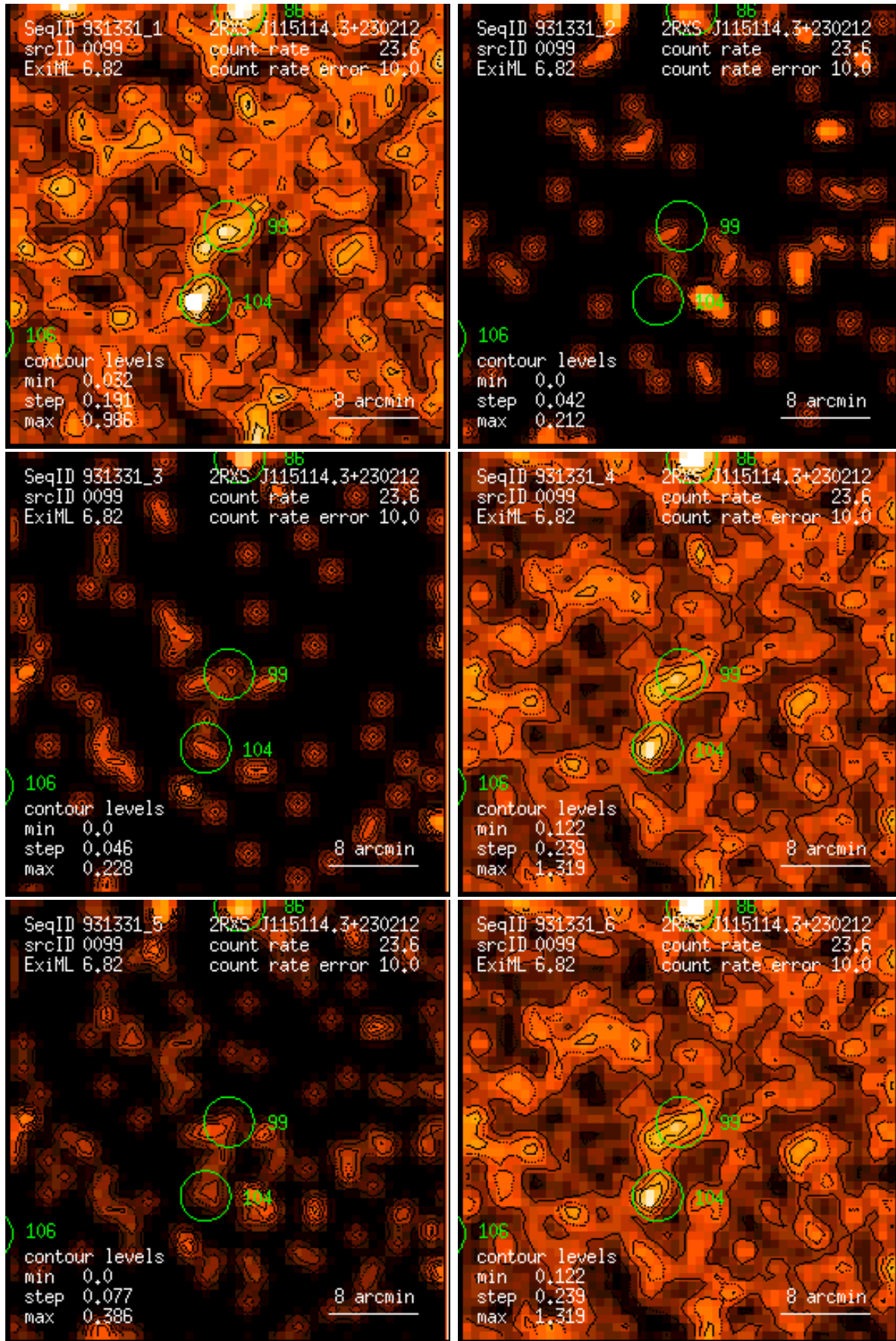
Figure 99: RASS 931331: detection 0099: band rate images, Gaussian filter: (1) PSPC channels 11 – 41, (2) 52 – 90, (3) 91 – 201, (4) 11 – 235, (5) 52 – 201, (6) 11 – 201. Broad band rates in counts/ks. Band rate contour levels in counts/ks/arcmin 2 .
