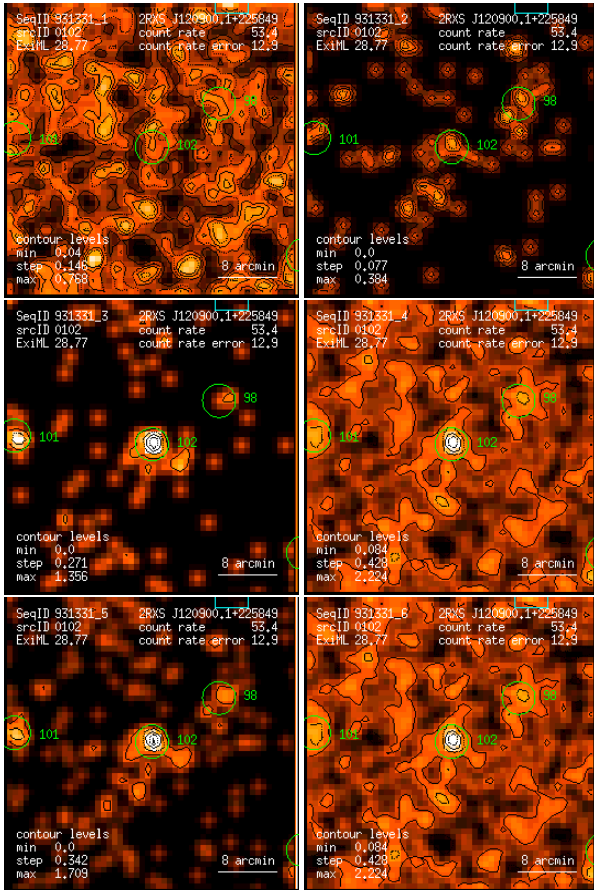
Figure 102: RASS 931331: detection 0102: band rate images, Gaussian filter: (1) PSPC channels 11 – 41, (2) 52 – 90, (3) 91 – 201, (4) 11 – 235, (5) 52 – 201, (6) 11 – 201. Broad band rates in counts/ks. Band rate contour levels in counts/ks/arcmin 2 .
