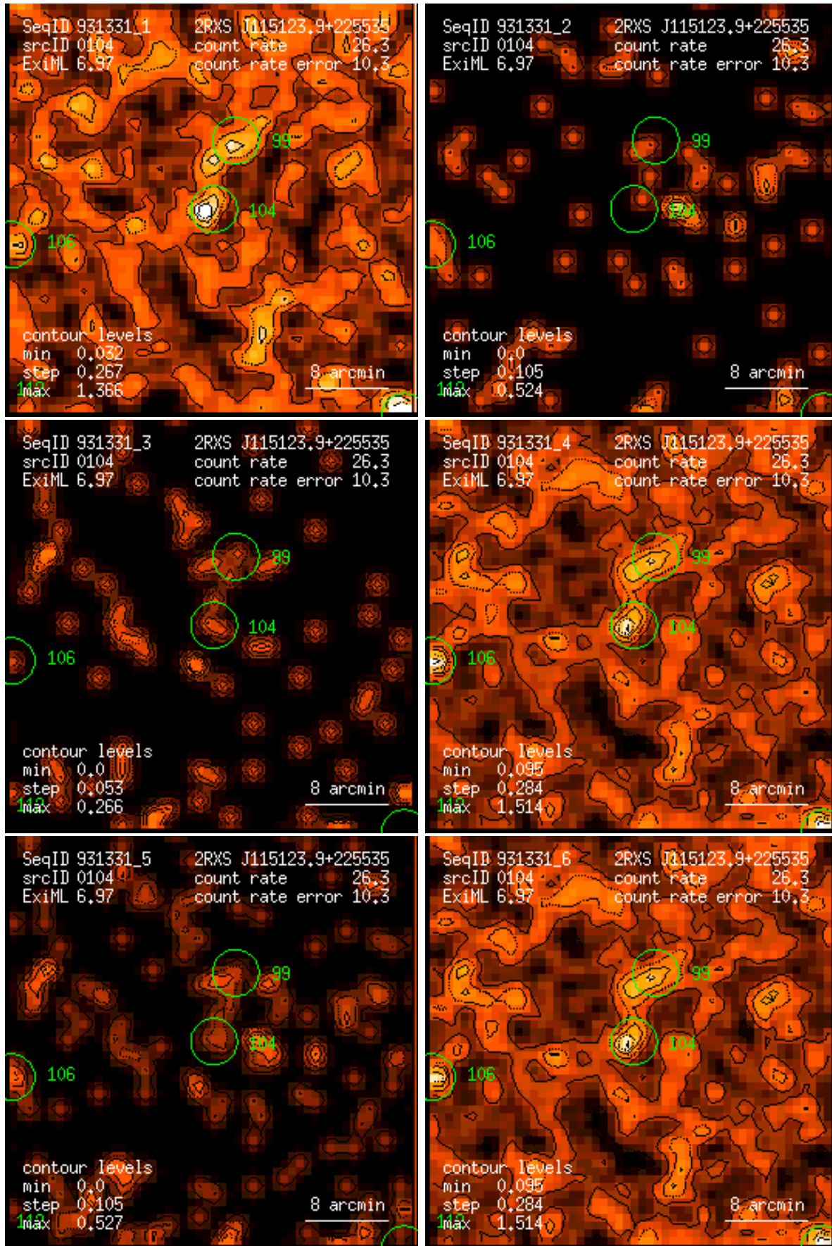
Figure 104: RASS 931331: detection 0104: band rate images, Gaussian filter: (1) PSPC channels 11 – 41, (2) 52 – 90, (3) 91 – 201, (4) 11 – 235, (5) 52 – 201, (6) 11 – 201. Broad band rates in counts/ks. Band rate contour levels in counts/ks/arcmin 2 .
