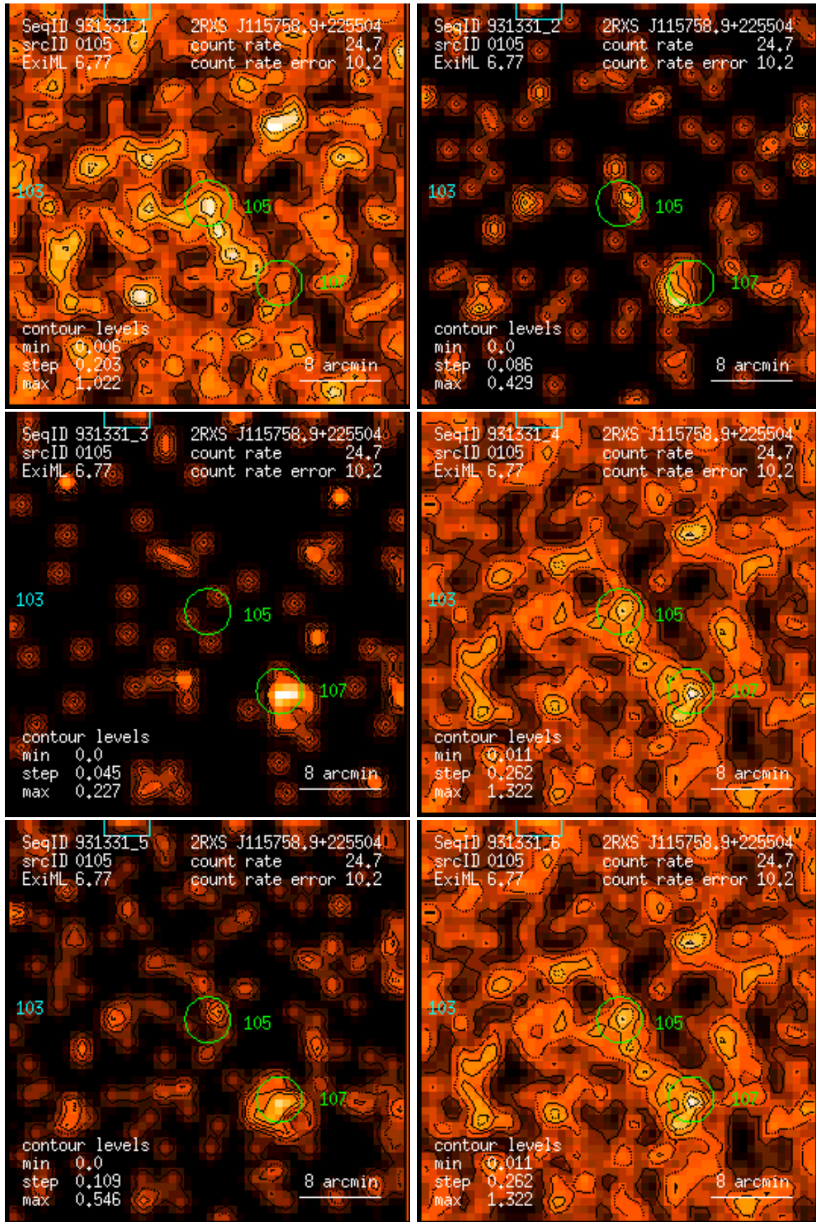
Figure 105: RASS 931331: detection 0105: band rate images, Gaussian filter: (1) PSPC channels 11 – 41, (2) 52 – 90, (3) 91 – 201, (4) 11 – 235, (5) 52 – 201, (6) 11 – 201. Broad band rates in counts/ks. Band rate contour levels in counts/ks/arcmin 2 .
