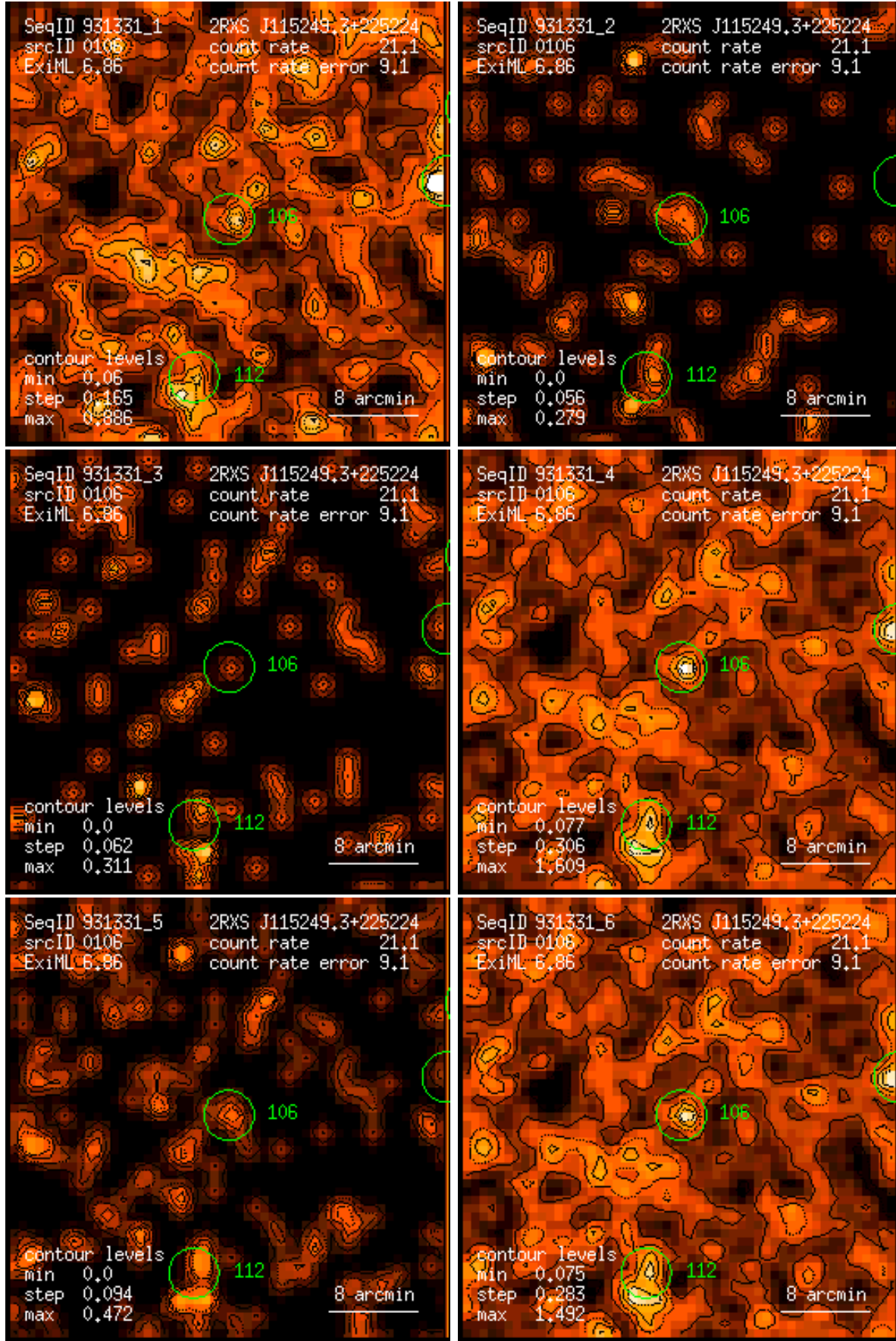
Figure 106: RASS 931331: detection 0106: band rate images, Gaussian filter: (1) PSPC channels 11 – 41, (2) 52 – 90, (3) 91 – 201, (4) 11 – 235, (5) 52 – 201, (6) 11 – 201. Broad band rates in counts/ks. Band rate contour levels in counts/ks/arcmin 2 .
