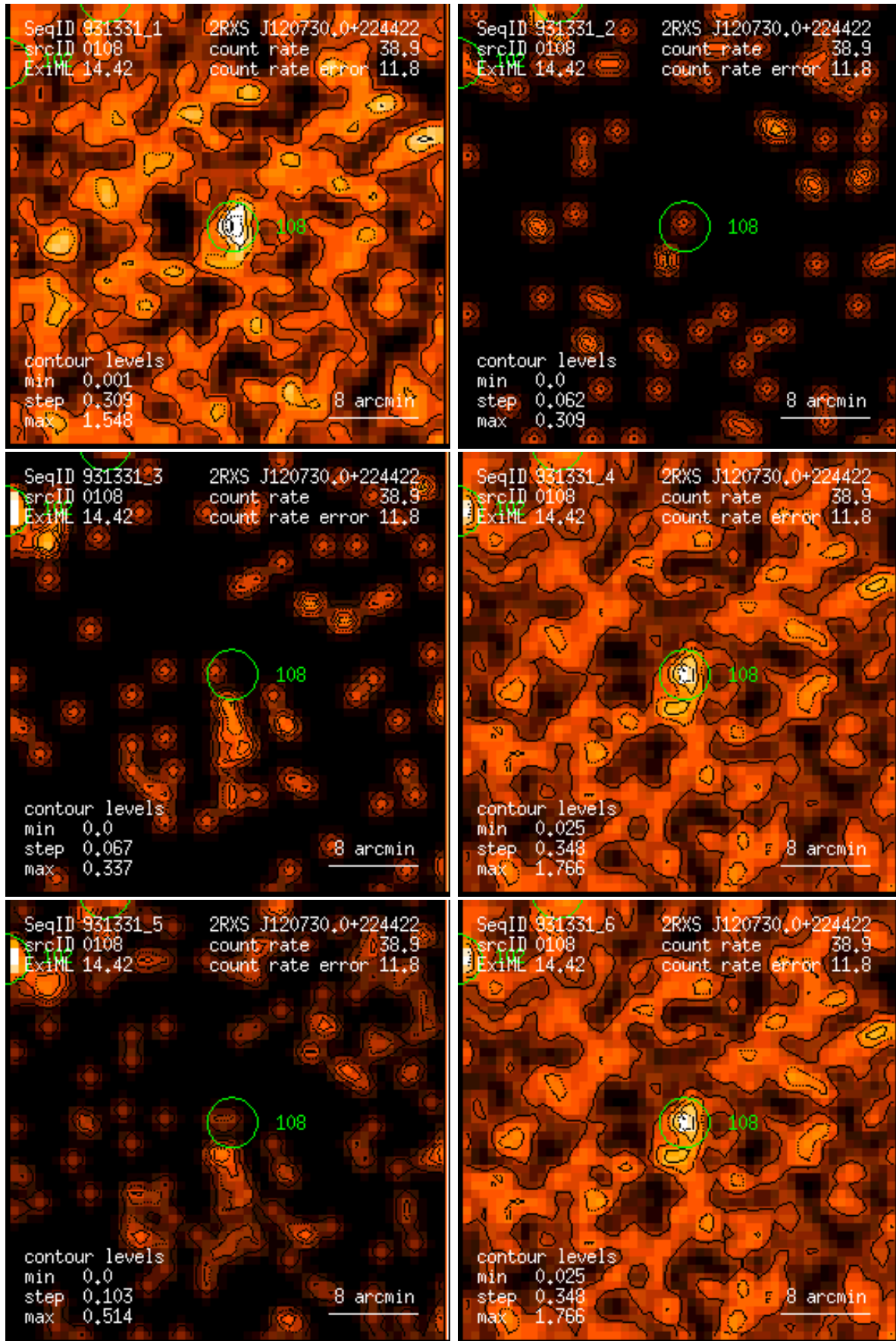
Figure 108: RASS 931331: detection 0108: band rate images, Gaussian filter: (1) PSPC channels 11 – 41, (2) 52 – 90, (3) 91 – 201, (4) 11 – 235, (5) 52 – 201, (6) 11 – 201. Broad band rates in counts/ks. Band rate contour levels in counts/ks/arcmin 2 .
