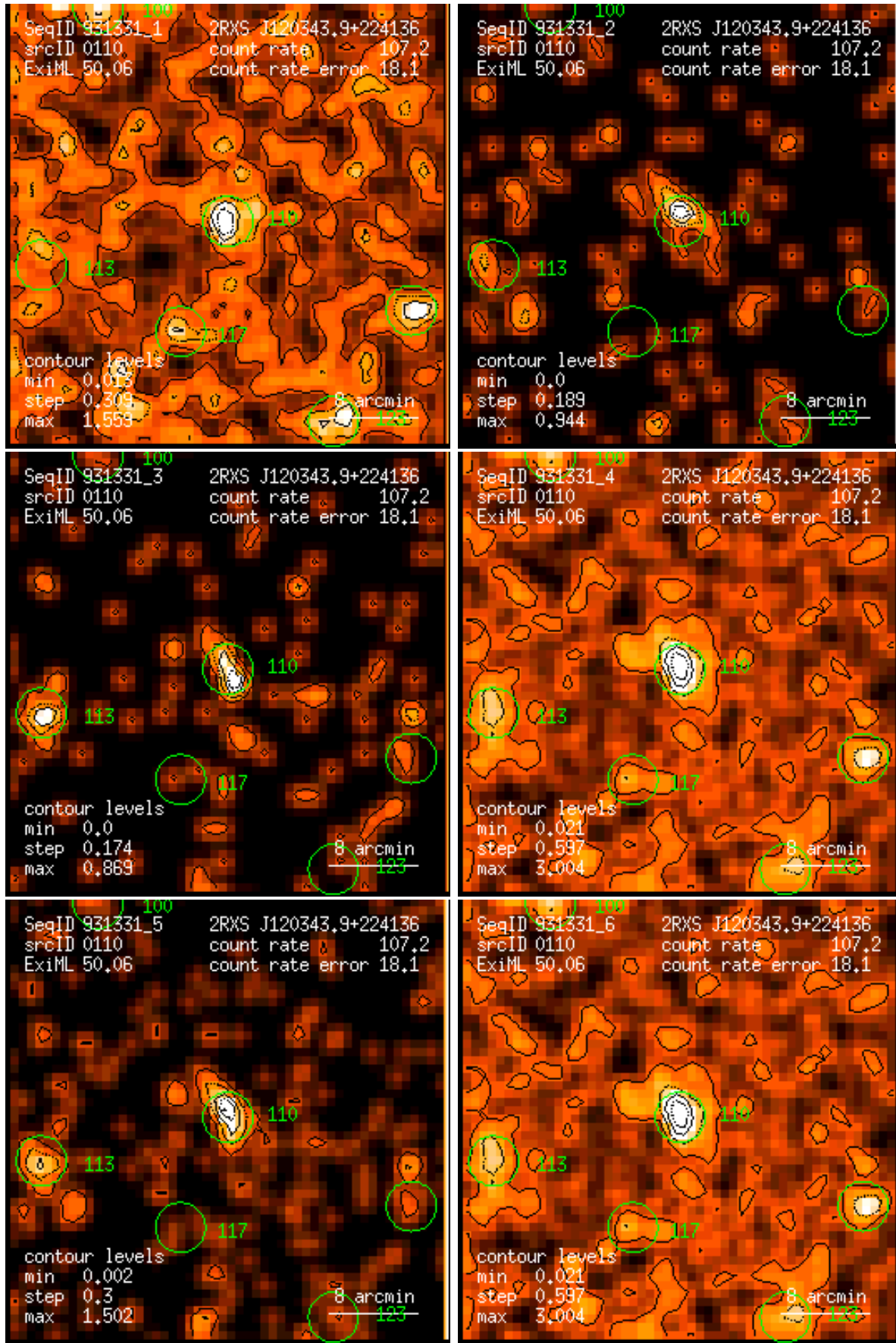
Figure 110: RASS 931331: detection 0110: band rate images, Gaussian filter: (1) PSPC channels 11 – 41, (2) 52 – 90, (3) 91 – 201, (4) 11 – 235, (5) 52 – 201, (6) 11 – 201. Broad band rates in counts/ks. Band rate contour levels in counts/ks/arcmin 2 .
