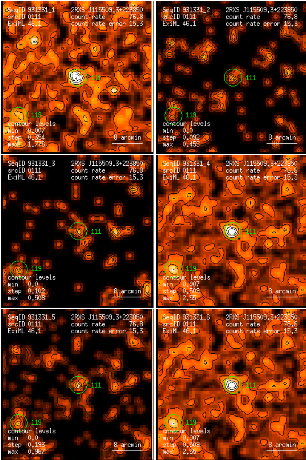
Figure 111: RASS 931331: detection 0111: band rate images, Gaussian filter: (1) PSPC channels 11 – 41, (2) 52 – 90, (3) 91 – 201, (4) 11 – 235, (5) 52 – 201, (6) 11 – 201. Broad band rates in counts/ks. Band rate contour levels in counts/ks/arcmin 2 .
