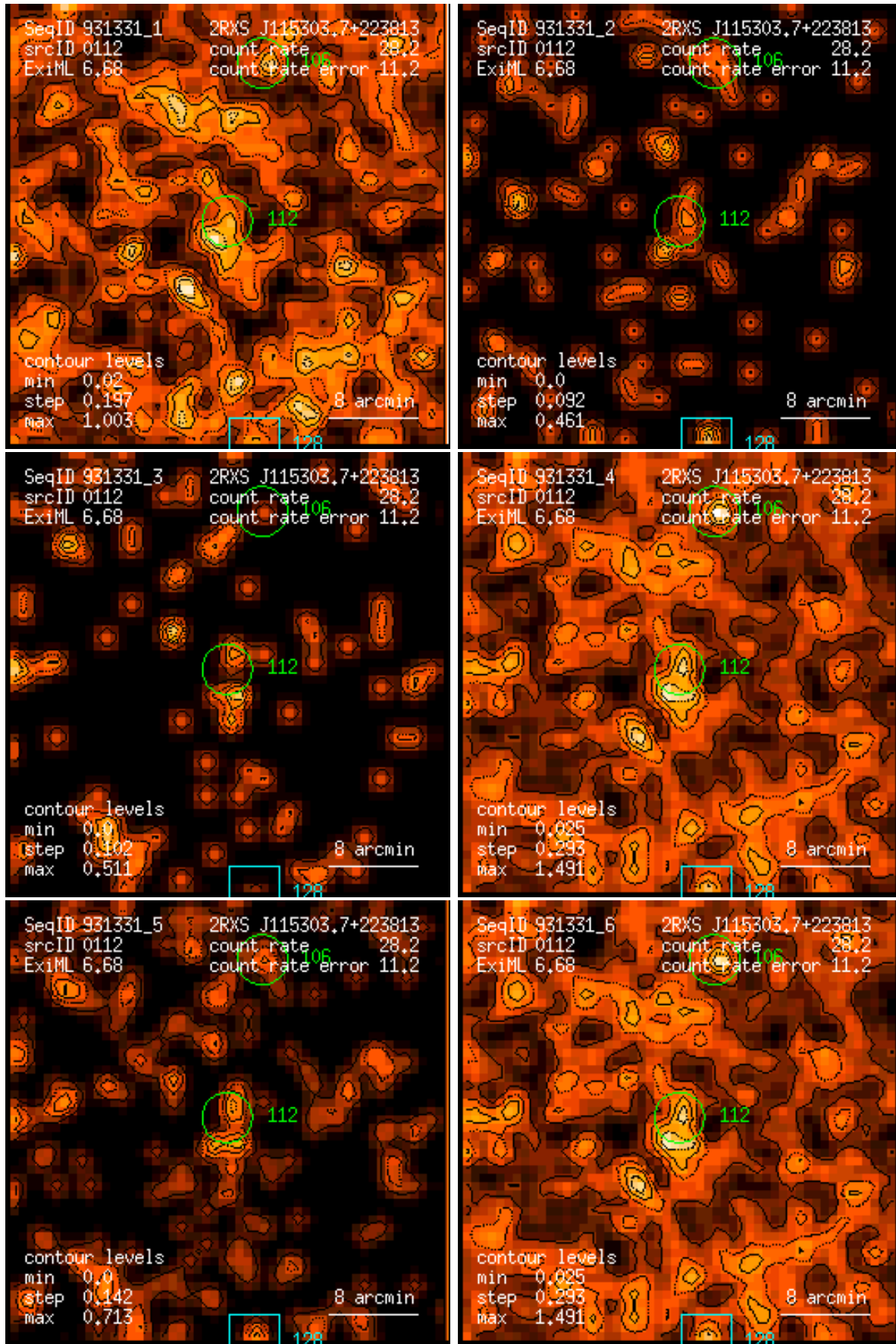
Figure 112: RASS 931331: detection 0112: band rate images, Gaussian filter: (1) PSPC channels 11 – 41, (2) 52 – 90, (3) 91 – 201, (4) 11 – 235, (5) 52 – 201, (6) 11 – 201. Broad band rates in counts/ks. Band rate contour levels in counts/ks/arcmin 2 .
