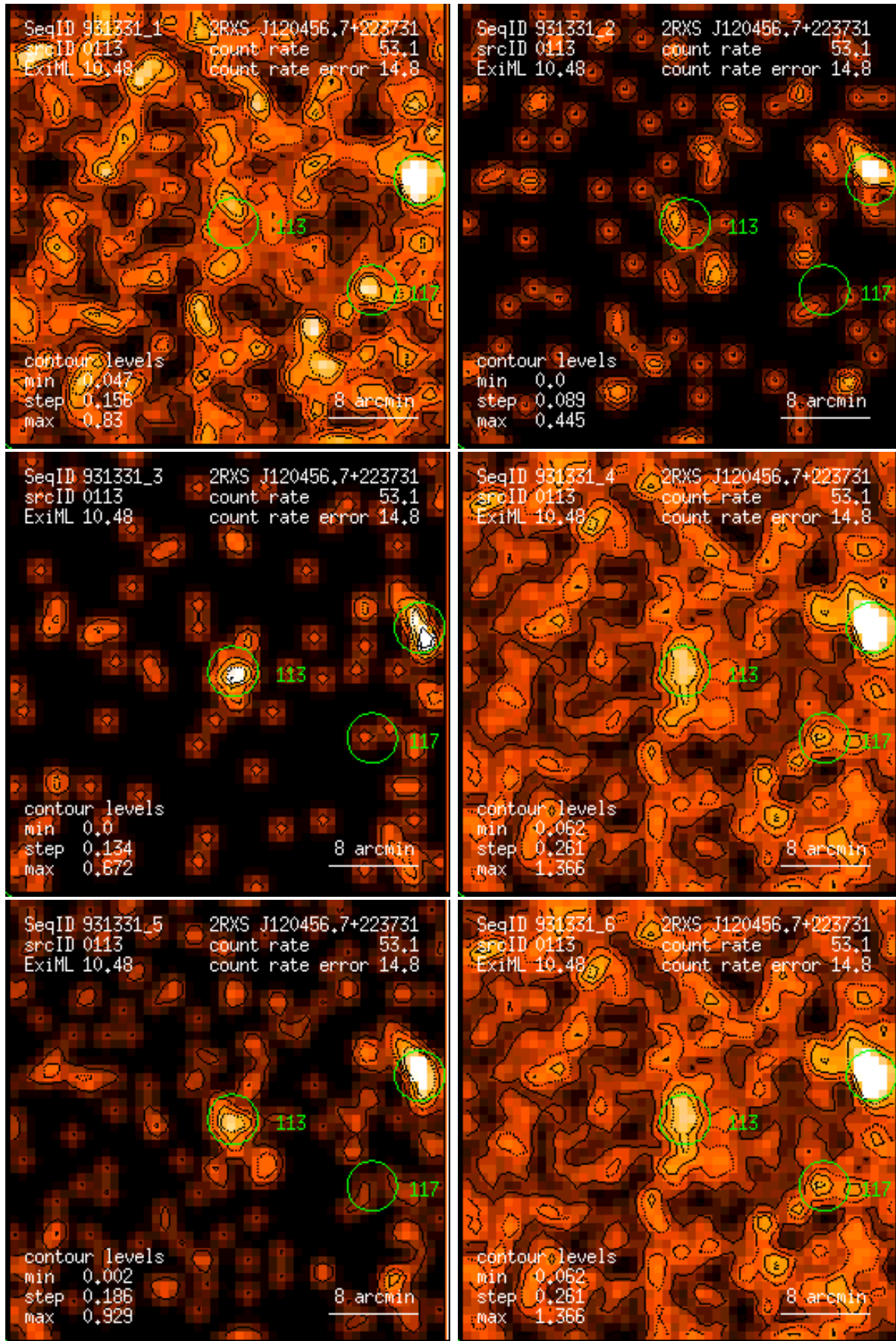
Figure 113: RASS 931331: detection 0113: band rate images, Gaussian filter: (1) PSPC channels 11 – 41, (2) 52 – 90, (3) 91 – 201, (4) 11 – 235, (5) 52 – 201, (6) 11 – 201. Broad band rates in counts/ks. Band rate contour levels in counts/ks/arcmin 2 .
