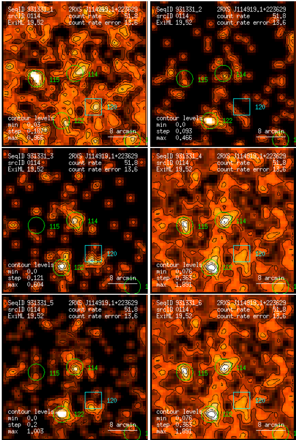
Figure 114: RASS 931331: detection 0114: band rate images, Gaussian filter: (1) PSPC channels 11 – 41, (2) 52 – 90, (3) 91 – 201, (4) 11 – 235, (5) 52 – 201, (6) 11 – 201. Broad band rates in counts/ks. Band rate contour levels in counts/ks/arcmin 2 .
