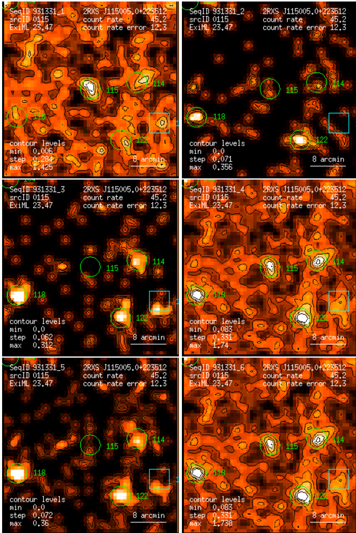
Figure 115: RASS 931331: detection 0115: band rate images, Gaussian filter: (1) PSPC channels 11 – 41, (2) 52 – 90, (3) 91 – 201, (4) 11 – 235, (5) 52 – 201, (6) 11 – 201. Broad band rates in counts/ks. Band rate contour levels in counts/ks/arcmin 2 .
