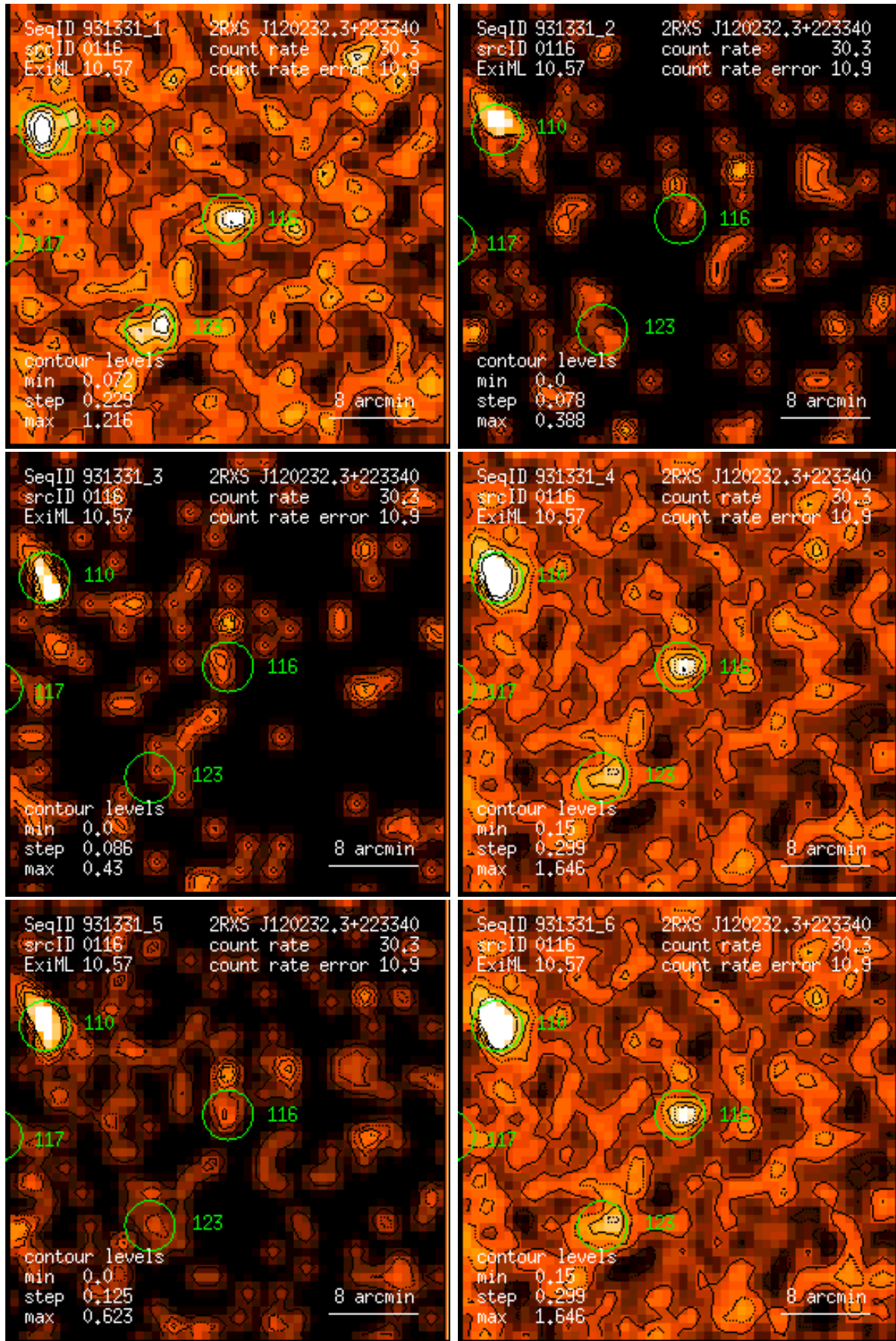
Figure 116: RASS 931331: detection 0116: band rate images, Gaussian filter: (1) PSPC channels 11 – 41, (2) 52 – 90, (3) 91 – 201, (4) 11 – 235, (5) 52 – 201, (6) 11 – 201. Broad band rates in counts/ks. Band rate contour levels in counts/ks/arcmin 2 .
