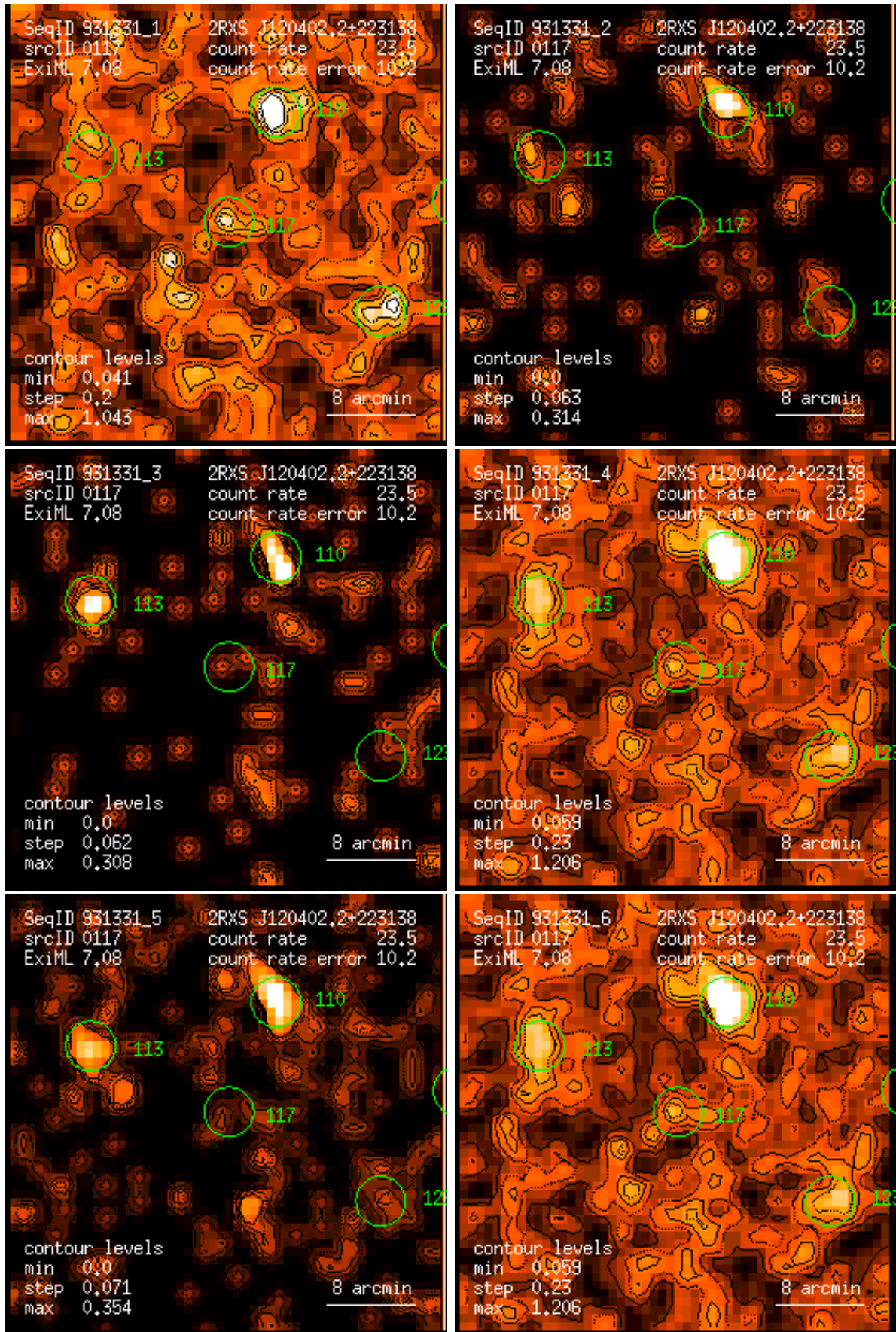
Figure 117: RASS 931331: detection 0117: band rate images, Gaussian filter: (1) PSPC channels 11 – 41, (2) 52 – 90, (3) 91 – 201, (4) 11 – 235, (5) 52 – 201, (6) 11 – 201. Broad band rates in counts/ks. Band rate contour levels in counts/ks/arcmin 2 .
