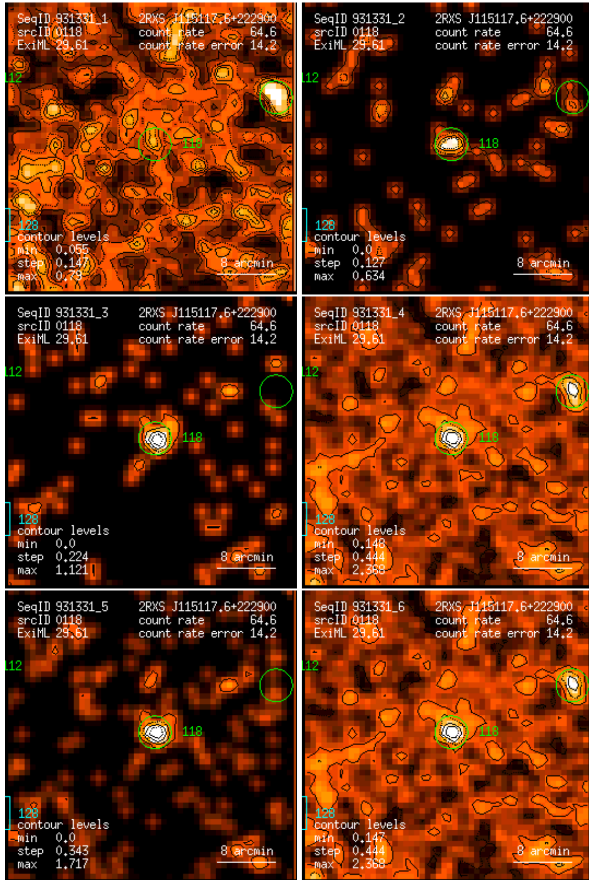
Figure 118: RASS 931331: detection 0118: band rate images, Gaussian filter: (1) PSPC channels 11 – 41, (2) 52 – 90, (3) 91 – 201, (4) 11 – 235, (5) 52 – 201, (6) 11 – 201. Broad band rates in counts/ks. Band rate contour levels in counts/ks/arcmin 2 .
