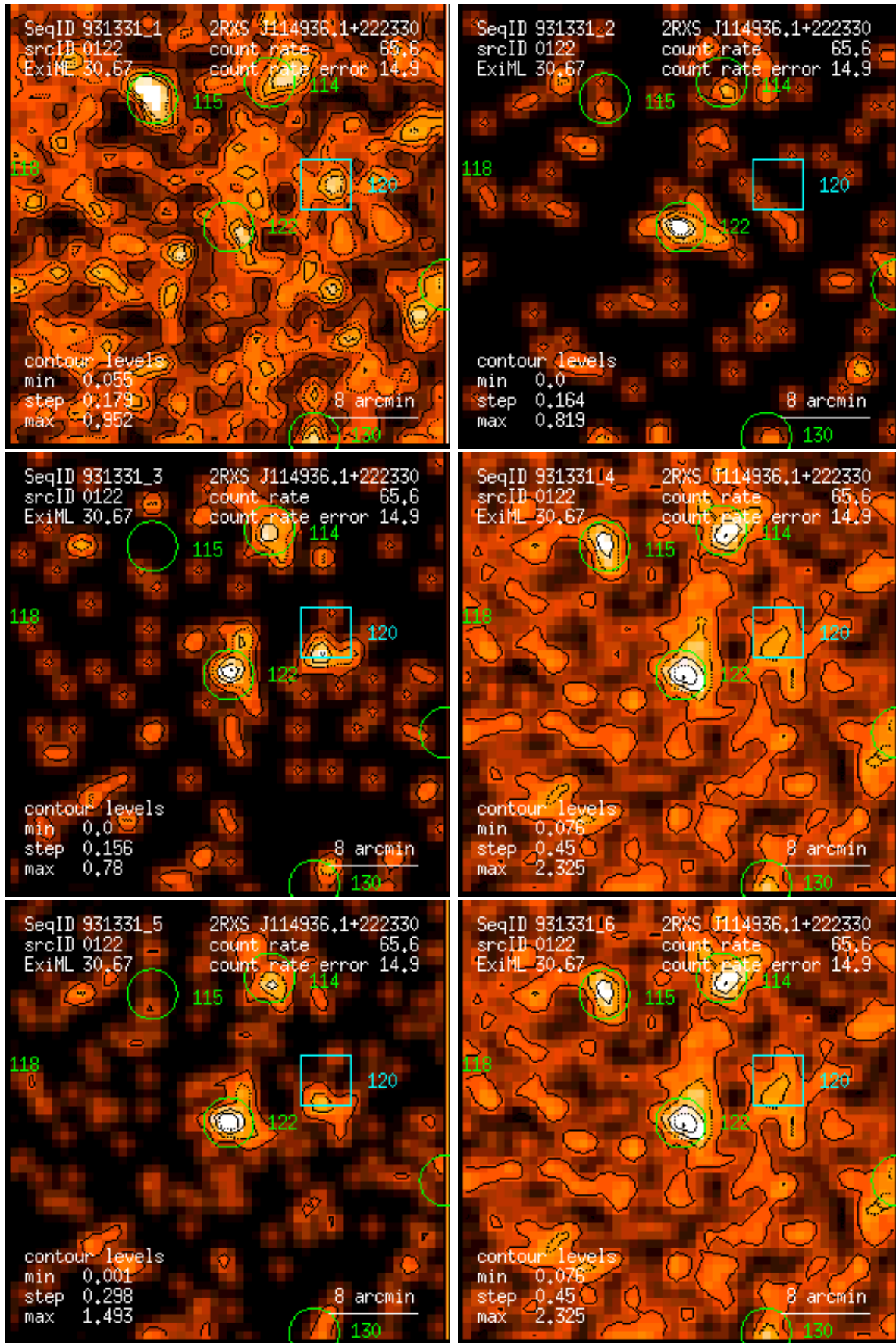
Figure 122: RASS 931331: detection 0122: band rate images, Gaussian filter: (1) PSPC channels 11 – 41, (2) 52 – 90, (3) 91 – 201, (4) 11 – 235, (5) 52 – 201, (6) 11 – 201. Broad band rates in counts/ks. Band rate contour levels in counts/ks/arcmin 2 .
