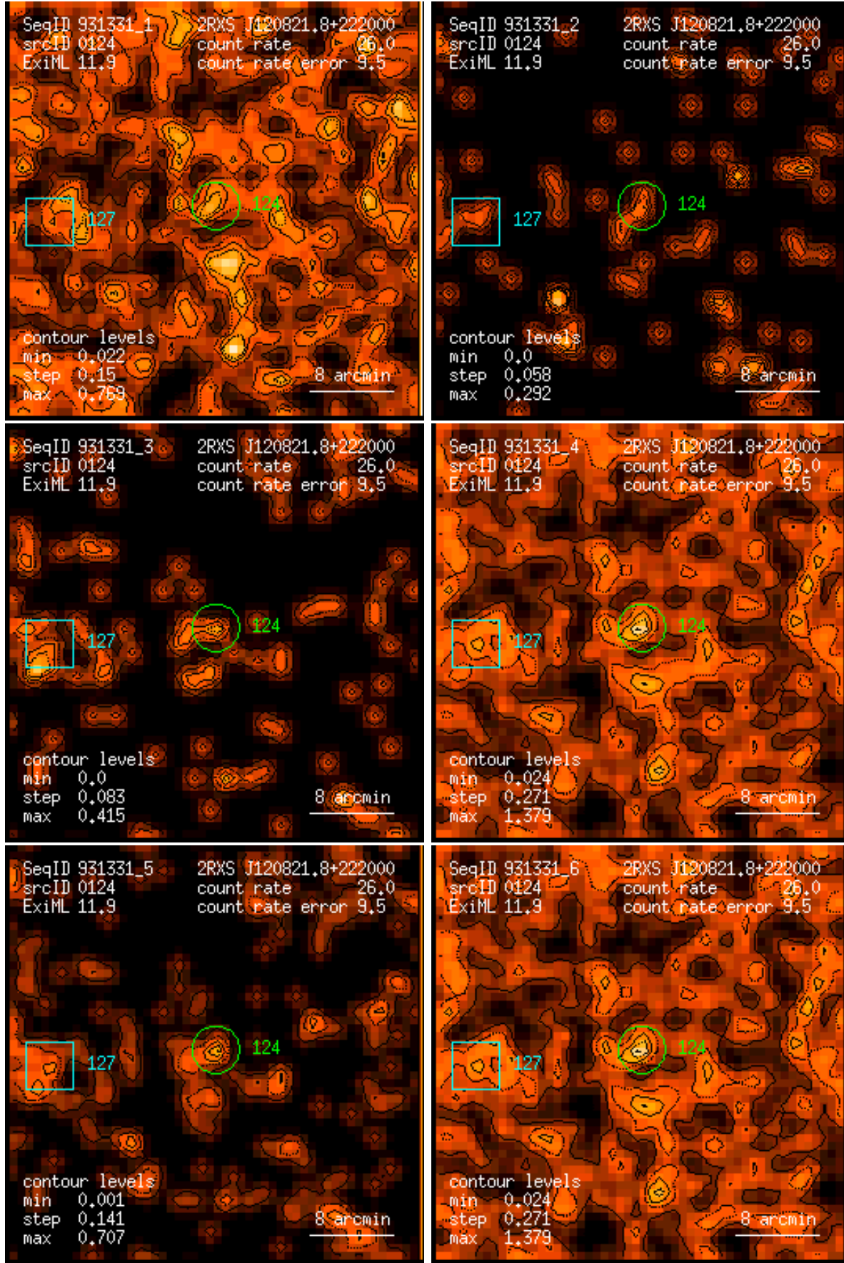
Figure 124: RASS 931331: detection 0124: band rate images, Gaussian filter: (1) PSPC channels 11 – 41, (2) 52 – 90, (3) 91 – 201, (4) 11 – 235, (5) 52 – 201, (6) 11 – 201. Broad band rates in counts/ks. Band rate contour levels in counts/ks/arcmin 2 .
