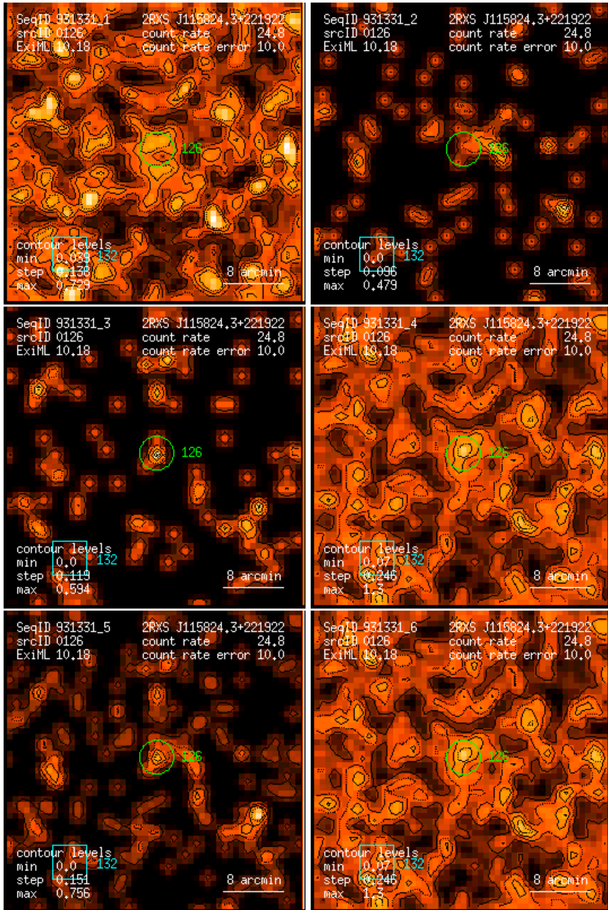
Figure 126: RASS 931331: detection 0126: band rate images, Gaussian filter: (1) PSPC channels 11 – 41, (2) 52 – 90, (3) 91 – 201, (4) 11 – 235, (5) 52 – 201, (6) 11 – 201. Broad band rates in counts/ks. Band rate contour levels in counts/ks/arcmin 2 .
