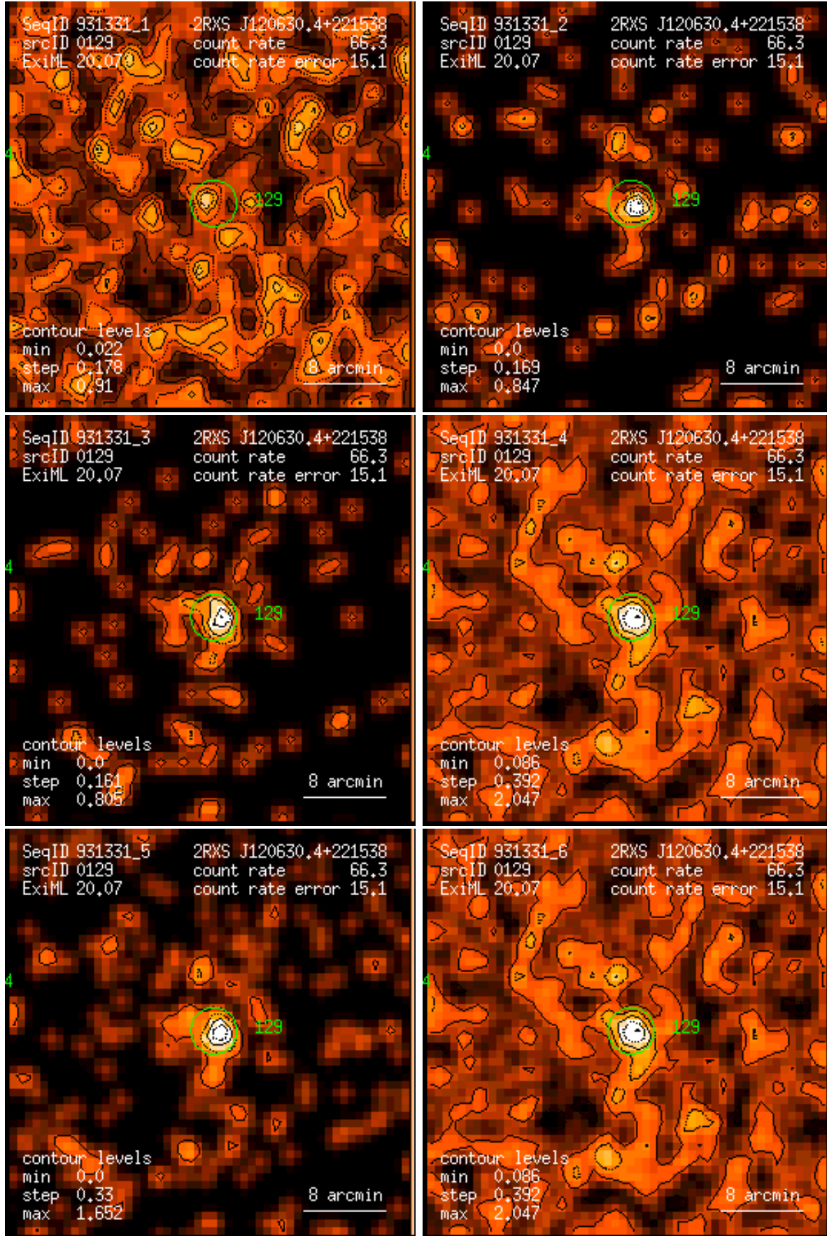
Figure 129: RASS 931331: detection 0129: band rate images, Gaussian filter: (1) PSPC channels 11 – 41, (2) 52 – 90, (3) 91 – 201, (4) 11 – 235, (5) 52 – 201, (6) 11 – 201. Broad band rates in counts/ks. Band rate contour levels in counts/ks/arcmin 2 .
