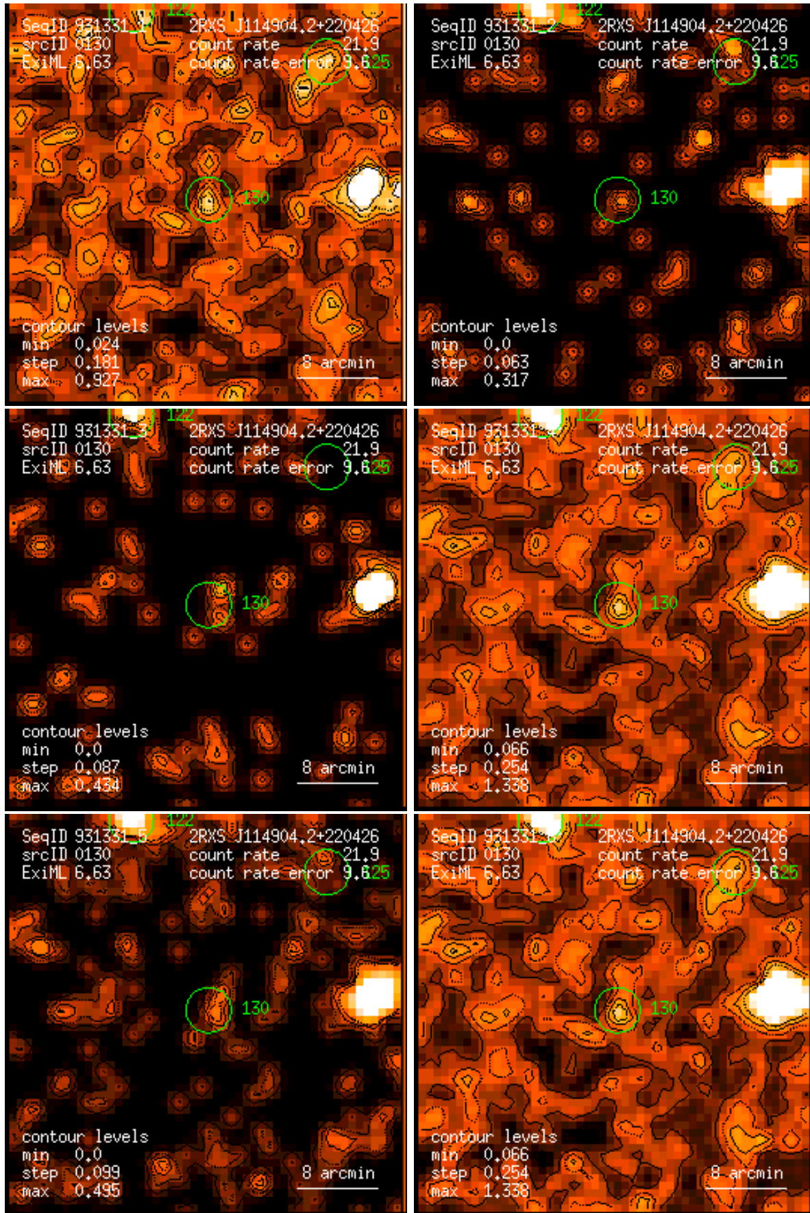
Figure 130: RASS 931331: detection 0130: band rate images, Gaussian filter: (1) PSPC channels 11 – 41, (2) 52 – 90, (3) 91 – 201, (4) 11 – 235, (5) 52 – 201, (6) 11 – 201. Broad band rates in counts/ks. Band rate contour levels in counts/ks/arcmin 2 .
