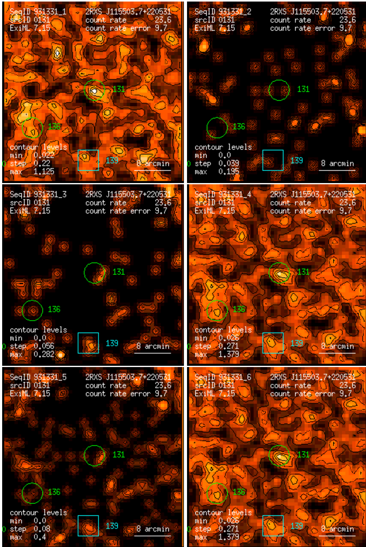
Figure 131: RASS 931331: detection 0131: band rate images, Gaussian filter: (1) PSPC channels 11 – 41, (2) 52 – 90, (3) 91 – 201, (4) 11 – 235, (5) 52 – 201, (6) 11 – 201. Broad band rates in counts/ks. Band rate contour levels in counts/ks/arcmin 2 .
