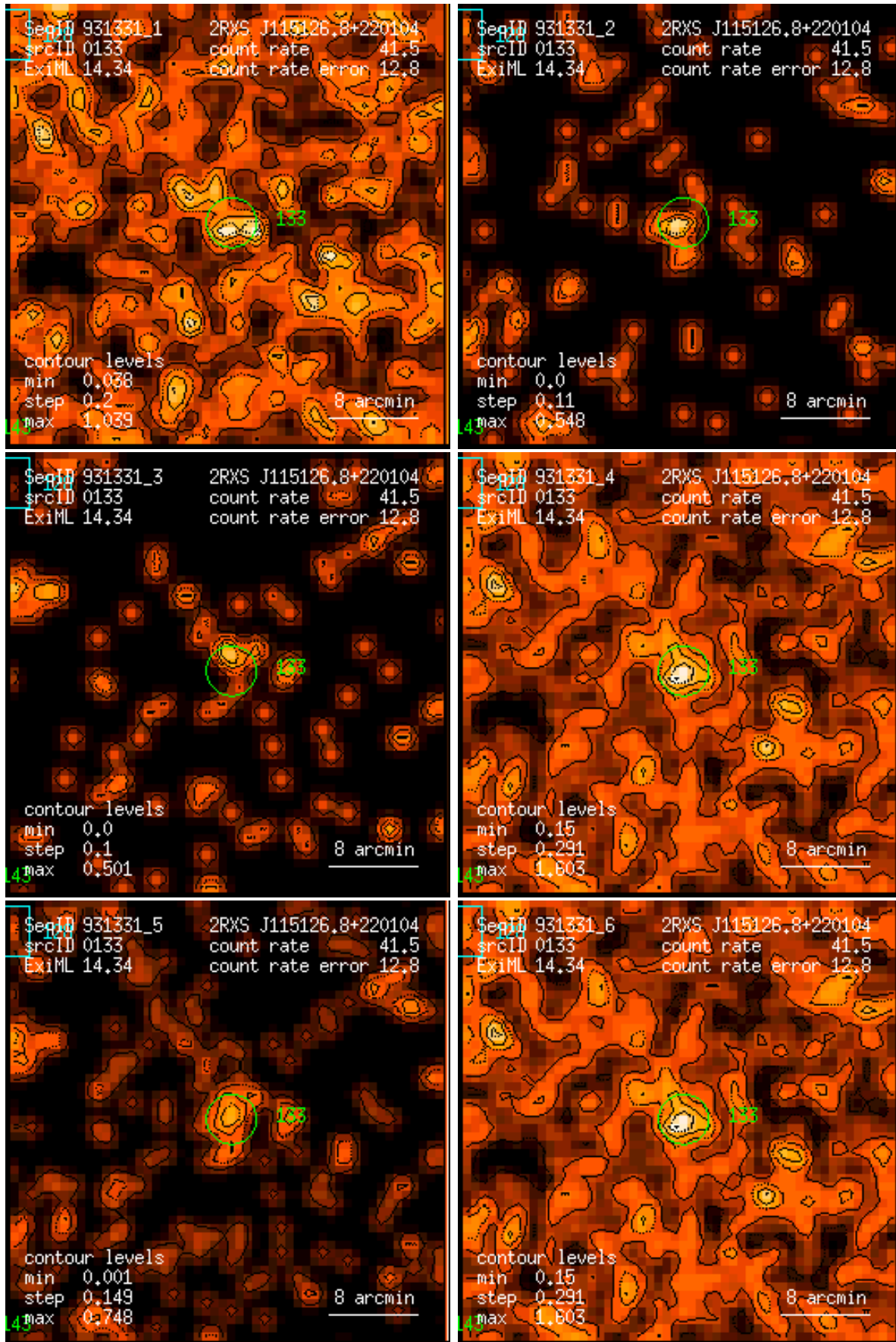
Figure 133: RASS 931331: detection 0133: band rate images, Gaussian filter: (1) PSPC channels 11 – 41, (2) 52 – 90, (3) 91 – 201, (4) 11 – 235, (5) 52 – 201, (6) 11 – 201. Broad band rates in counts/ks. Band rate contour levels in counts/ks/arcmin 2 .
