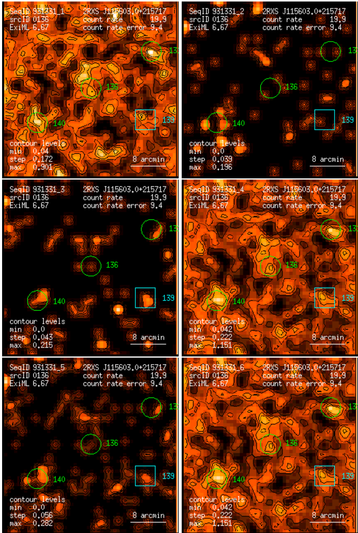
Figure 136: RASS 931331: detection 0136: band rate images, Gaussian filter: (1) PSPC channels 11 – 41, (2) 52 – 90, (3) 91 – 201, (4) 11 – 235, (5) 52 – 201, (6) 11 – 201. Broad band rates in counts/ks. Band rate contour levels in counts/ks/arcmin 2 .
