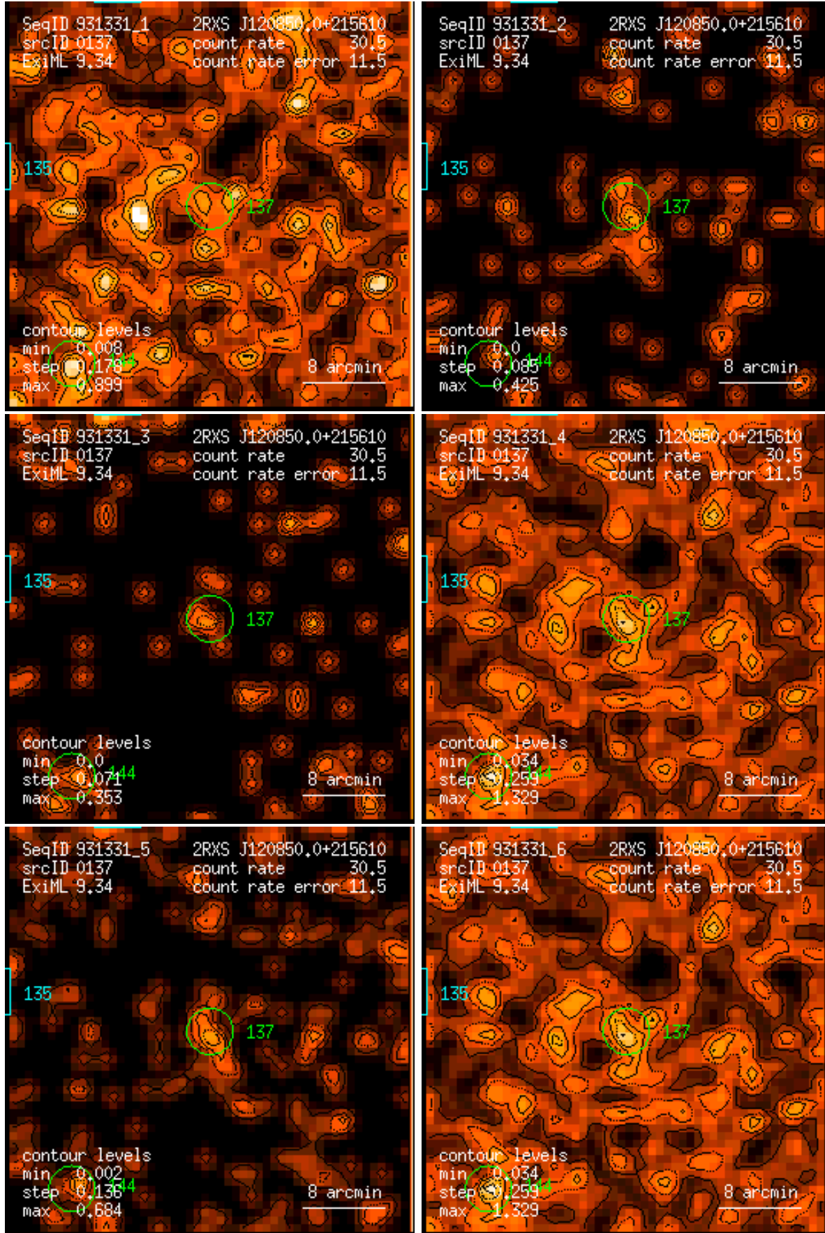
Figure 137: RASS 931331: detection 0137: band rate images, Gaussian filter: (1) PSPC channels 11 – 41, (2) 52 – 90, (3) 91 – 201, (4) 11 – 235, (5) 52 – 201, (6) 11 – 201. Broad band rates in counts/ks. Band rate contour levels in counts/ks/arcmin 2 .
