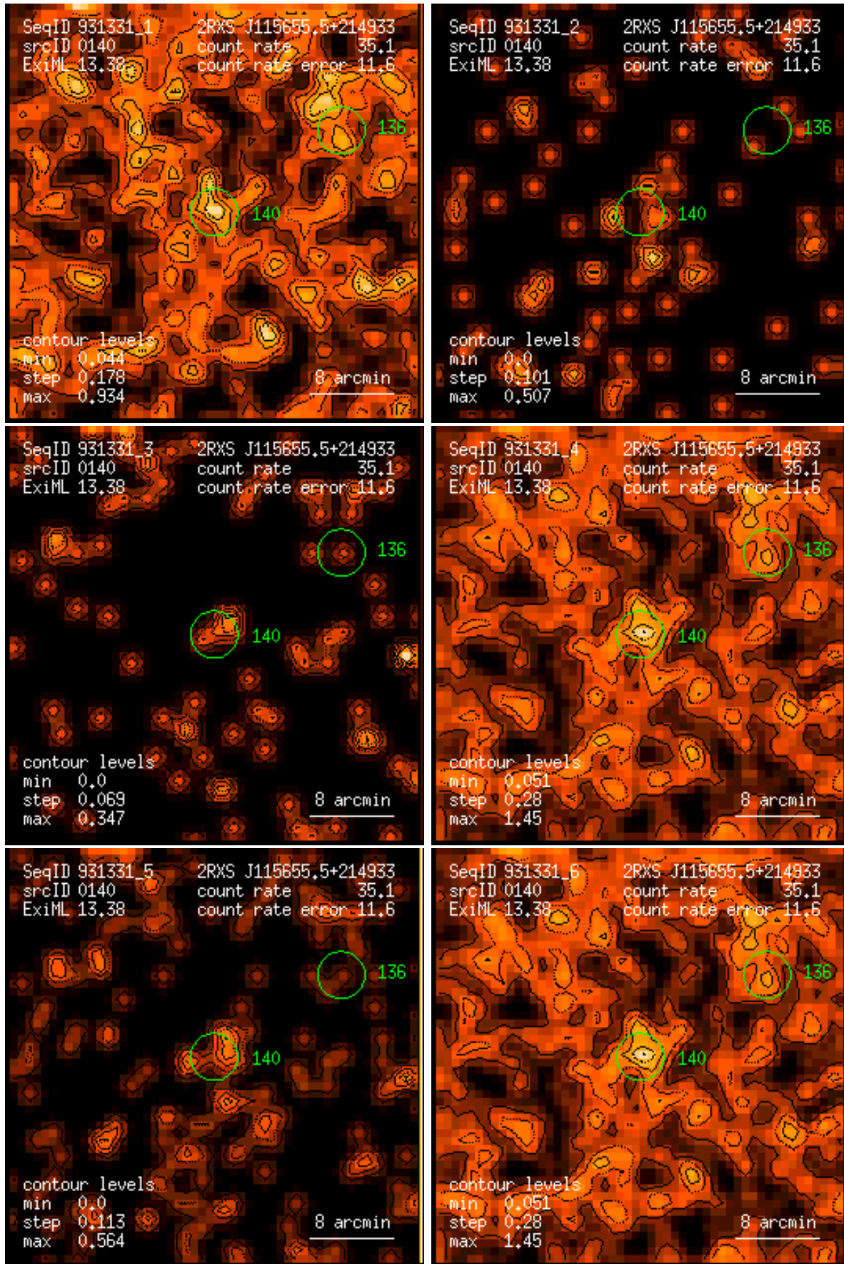
Figure 140: RASS 931331: detection 0140: band rate images, Gaussian filter: (1) PSPC channels 11 – 41, (2) 52 – 90, (3) 91 – 201, (4) 11 – 235, (5) 52 – 201, (6) 11 – 201. Broad band rates in counts/ks. Band rate contour levels in counts/ks/arcmin 2 .
