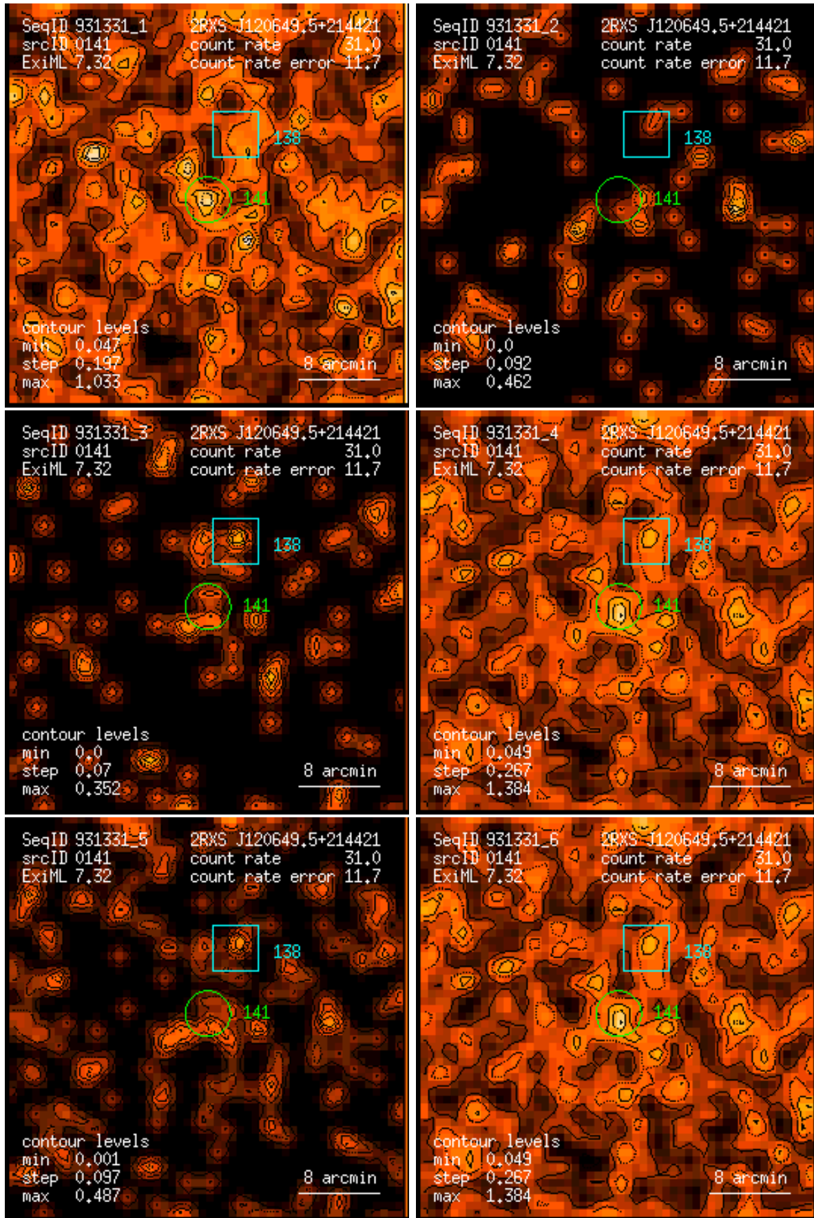
Figure 141: RASS 931331: detection 0141: band rate images, Gaussian filter: (1) PSPC channels 11 – 41, (2) 52 – 90, (3) 91 – 201, (4) 11 – 235, (5) 52 – 201, (6) 11 – 201. Broad band rates in counts/ks. Band rate contour levels in counts/ks/arcmin 2 .
