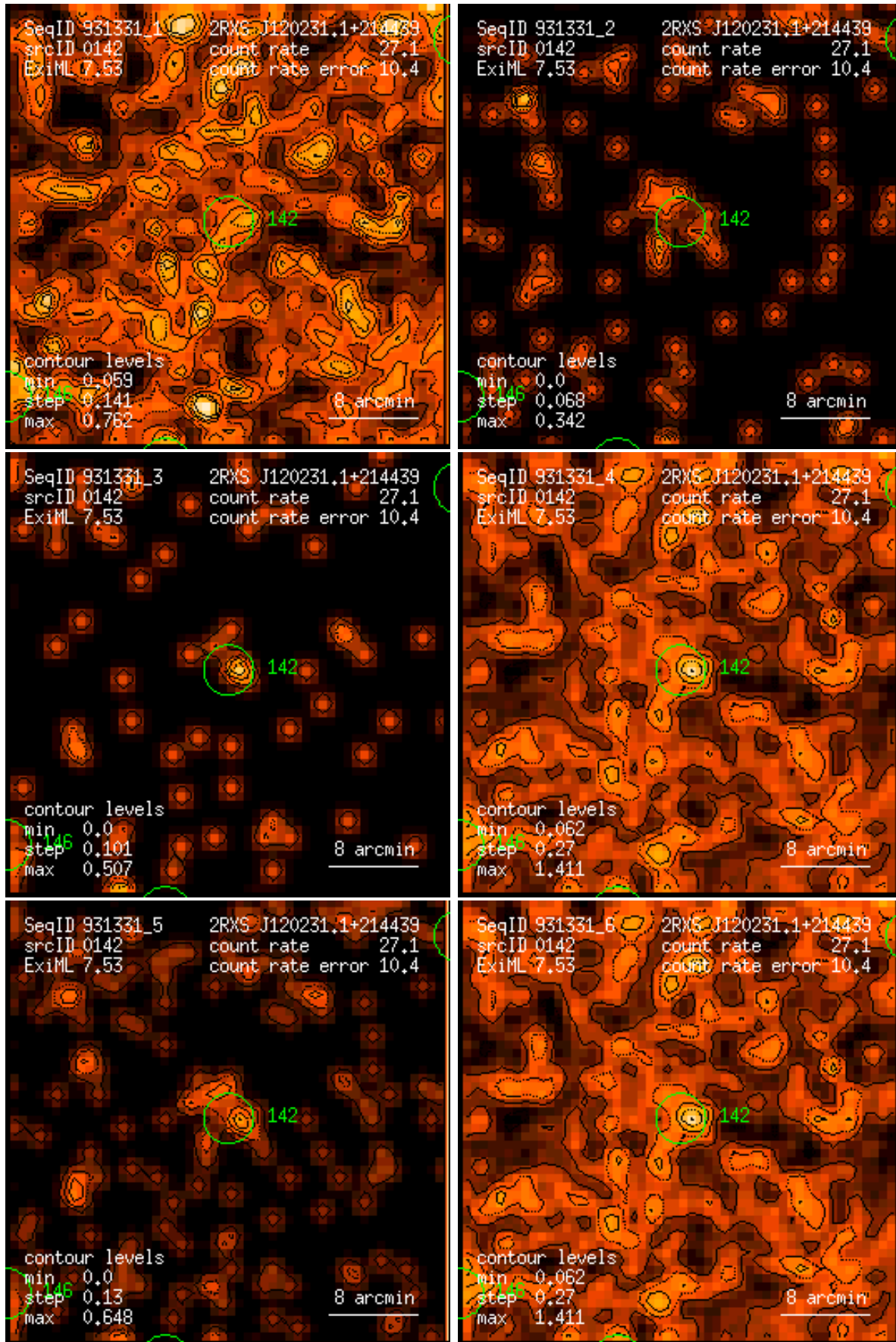
Figure 142: RASS 931331: detection 0142: band rate images, Gaussian filter: (1) PSPC channels 11 – 41, (2) 52 – 90, (3) 91 – 201, (4) 11 – 235, (5) 52 – 201, (6) 11 – 201. Broad band rates in counts/ks. Band rate contour levels in counts/ks/arcmin 2 .
