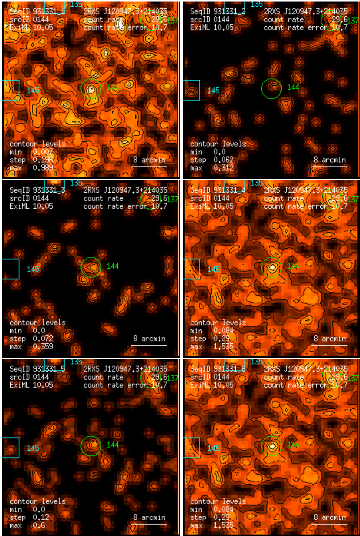
Figure 144: RASS 931331: detection 0144: band rate images, Gaussian filter: (1) PSPC channels 11 – 41, (2) 52 – 90, (3) 91 – 201, (4) 11 – 235, (5) 52 – 201, (6) 11 – 201. Broad band rates in counts/ks. Band rate contour levels in counts/ks/arcmin 2 .
