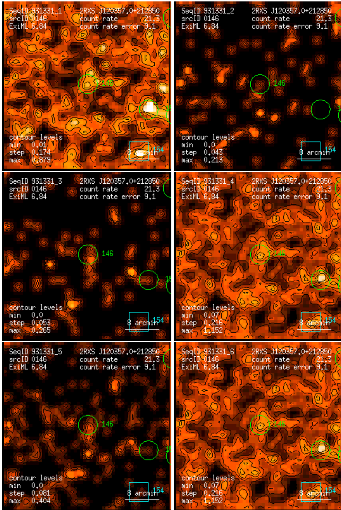
Figure 146: RASS 931331: detection 0146: band rate images, Gaussian filter: (1) PSPC channels 11 – 41, (2) 52 – 90, (3) 91 – 201, (4) 11 – 235, (5) 52 – 201, (6) 11 – 201. Broad band rates in counts/ks. Band rate contour levels in counts/ks/arcmin 2 .
