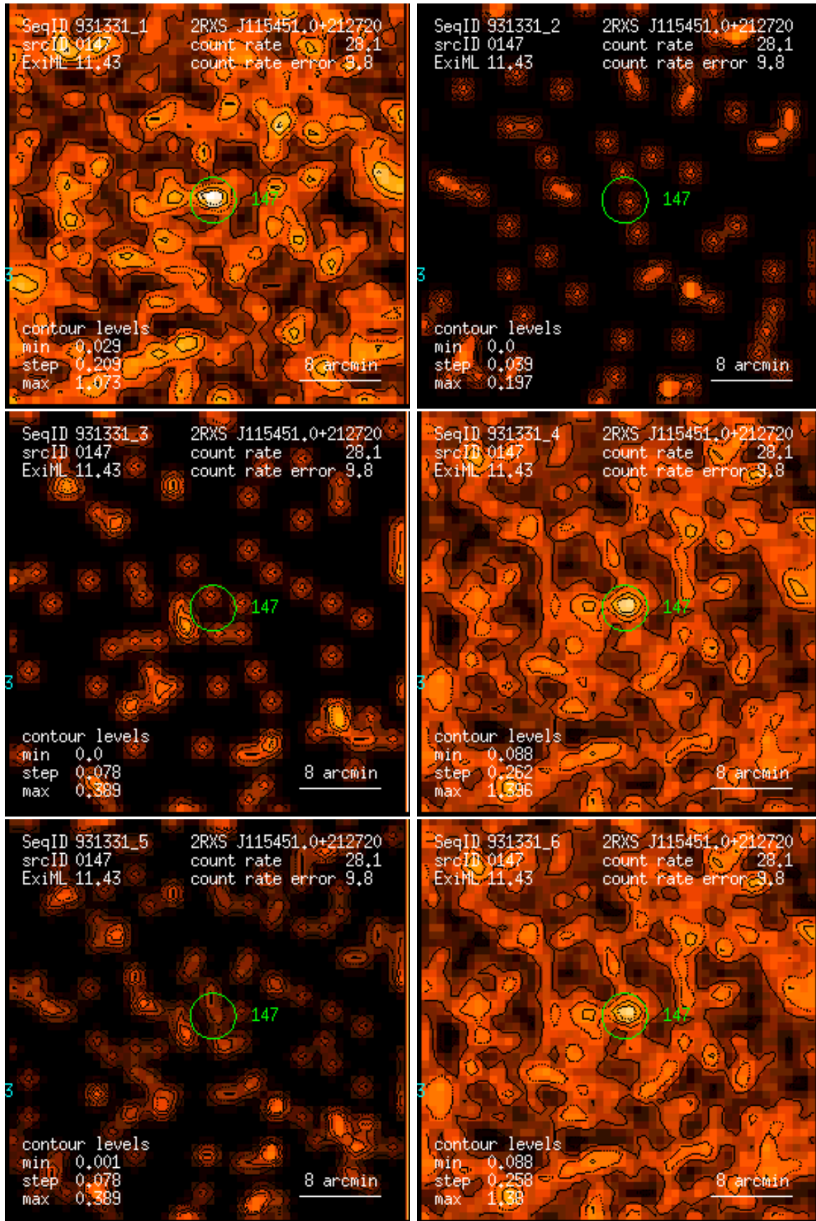
Figure 147: RASS 931331: detection 0147: band rate images, Gaussian filter: (1) PSPC channels 11 – 41, (2) 52 – 90, (3) 91 – 201, (4) 11 – 235, (5) 52 – 201, (6) 11 – 201. Broad band rates in counts/ks. Band rate contour levels in counts/ks/arcmin 2 .
