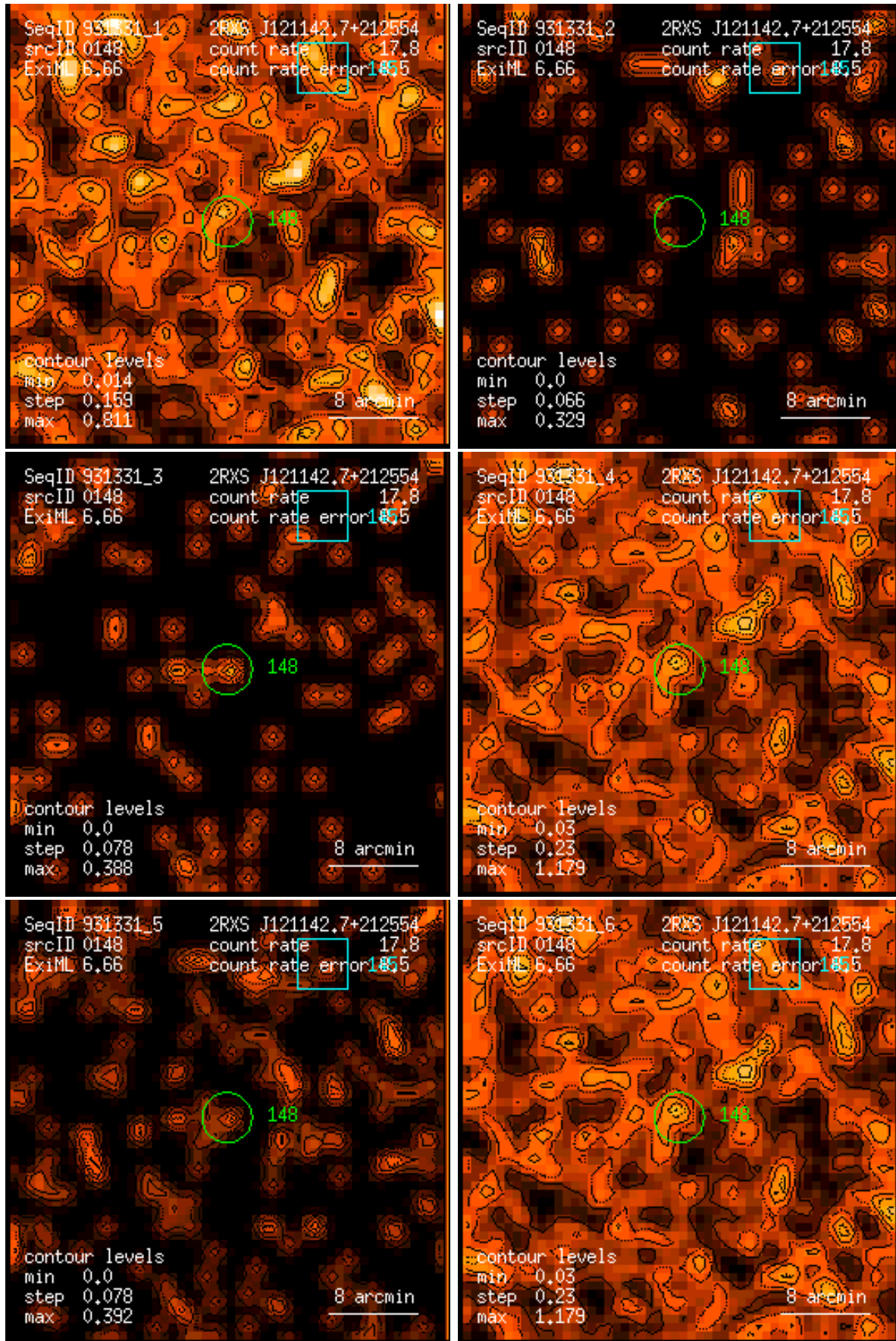
Figure 148: RASS 931331: detection 0148: band rate images, Gaussian filter: (1) PSPC channels 11 – 41, (2) 52 – 90, (3) 91 – 201, (4) 11 – 235, (5) 52 – 201, (6) 11 – 201. Broad band rates in counts/ks. Band rate contour levels in counts/ks/arcmin 2 .
