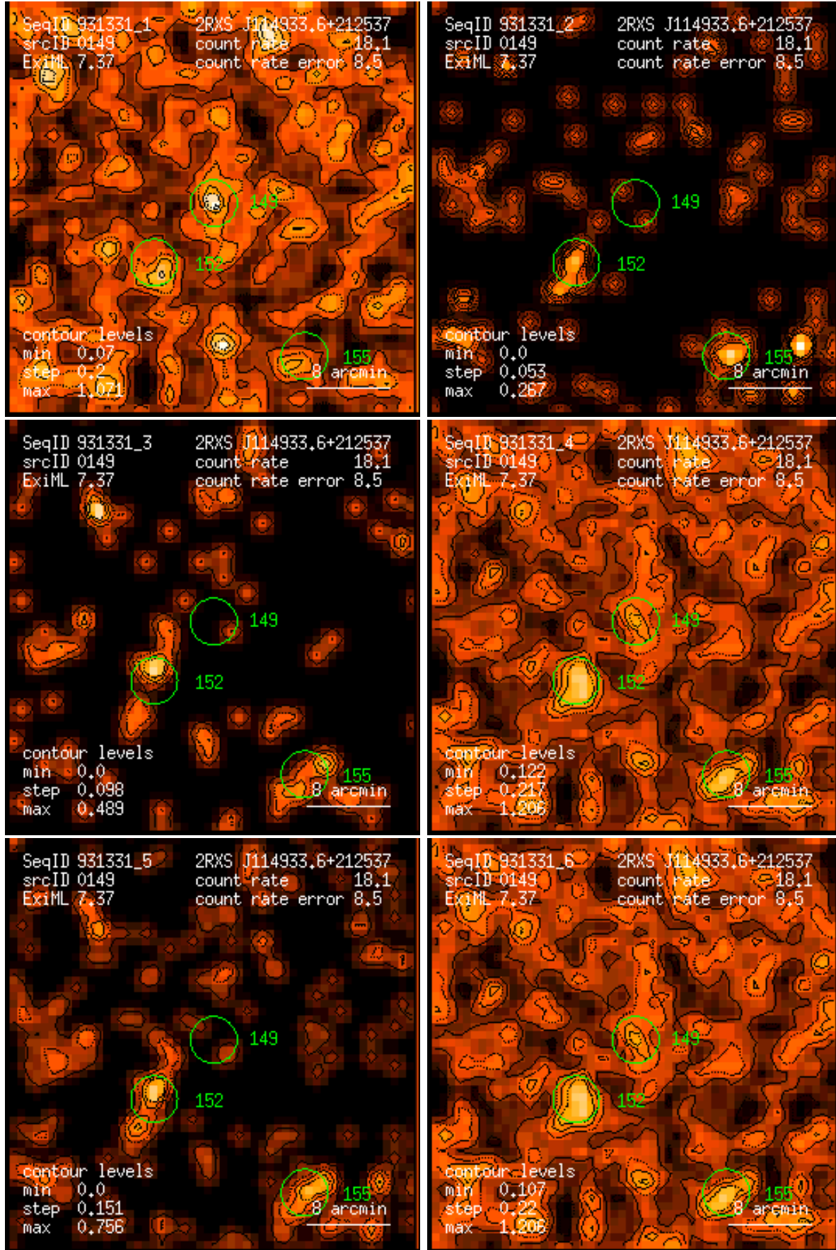
Figure 149: RASS 931331: detection 0149: band rate images, Gaussian filter: (1) PSPC channels 11 – 41, (2) 52 – 90, (3) 91 – 201, (4) 11 – 235, (5) 52 – 201, (6) 11 – 201. Broad band rates in counts/ks. Band rate contour levels in counts/ks/arcmin 2 .
