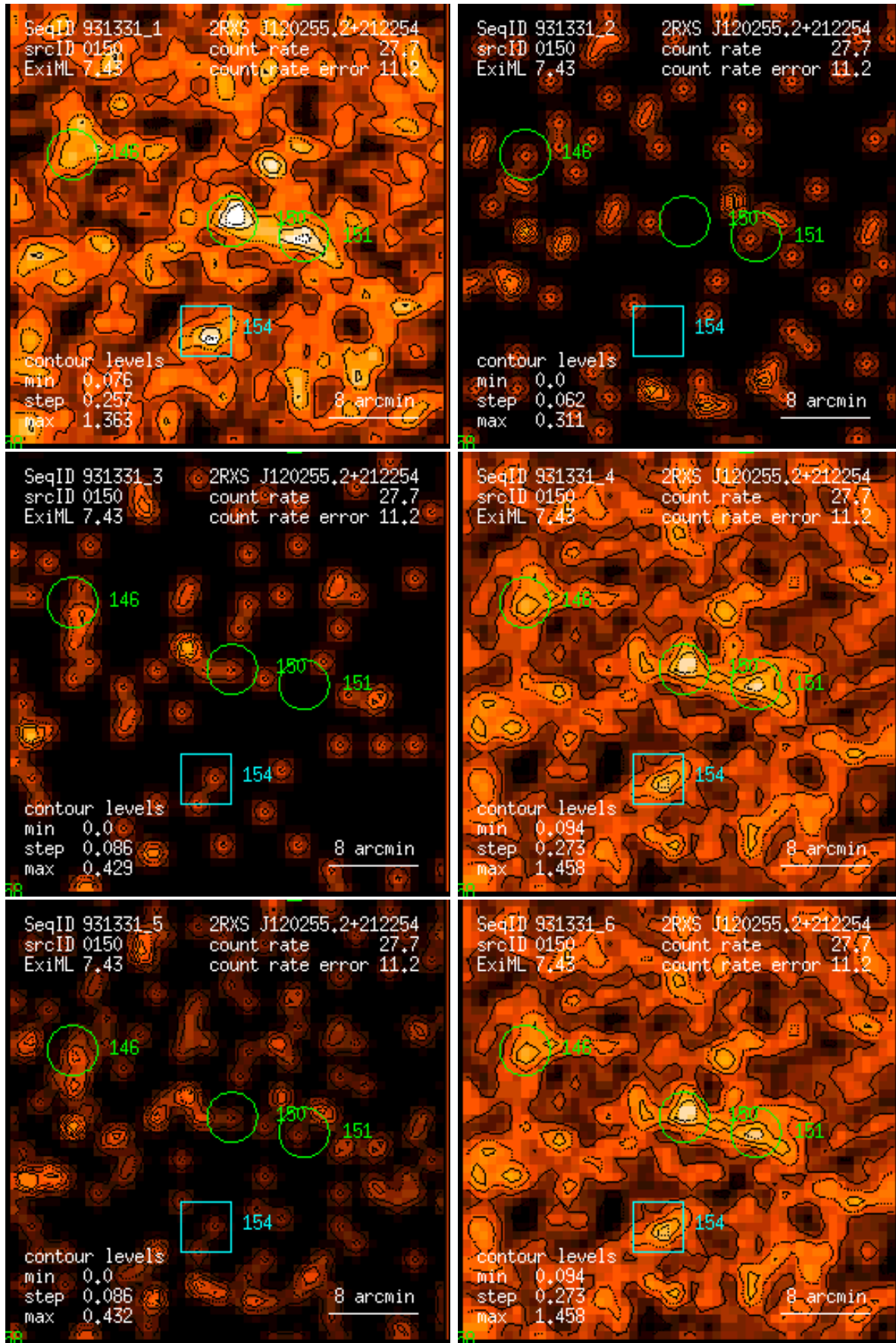
Figure 150: RASS 931331: detection 0150: band rate images, Gaussian filter: (1) PSPC channels 11 – 41, (2) 52 – 90, (3) 91 – 201, (4) 11 – 235, (5) 52 – 201, (6) 11 – 201. Broad band rates in counts/ks. Band rate contour levels in counts/ks/arcmin 2 .
