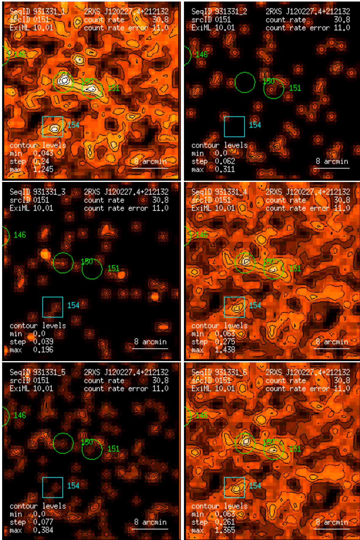
Figure 151: RASS 931331: detection 0151: band rate images, Gaussian filter: (1) PSPC channels 11 – 41, (2) 52 – 90, (3) 91 – 201, (4) 11 – 235, (5) 52 – 201, (6) 11 – 201. Broad band rates in counts/ks. Band rate contour levels in counts/ks/arcmin 2 .
