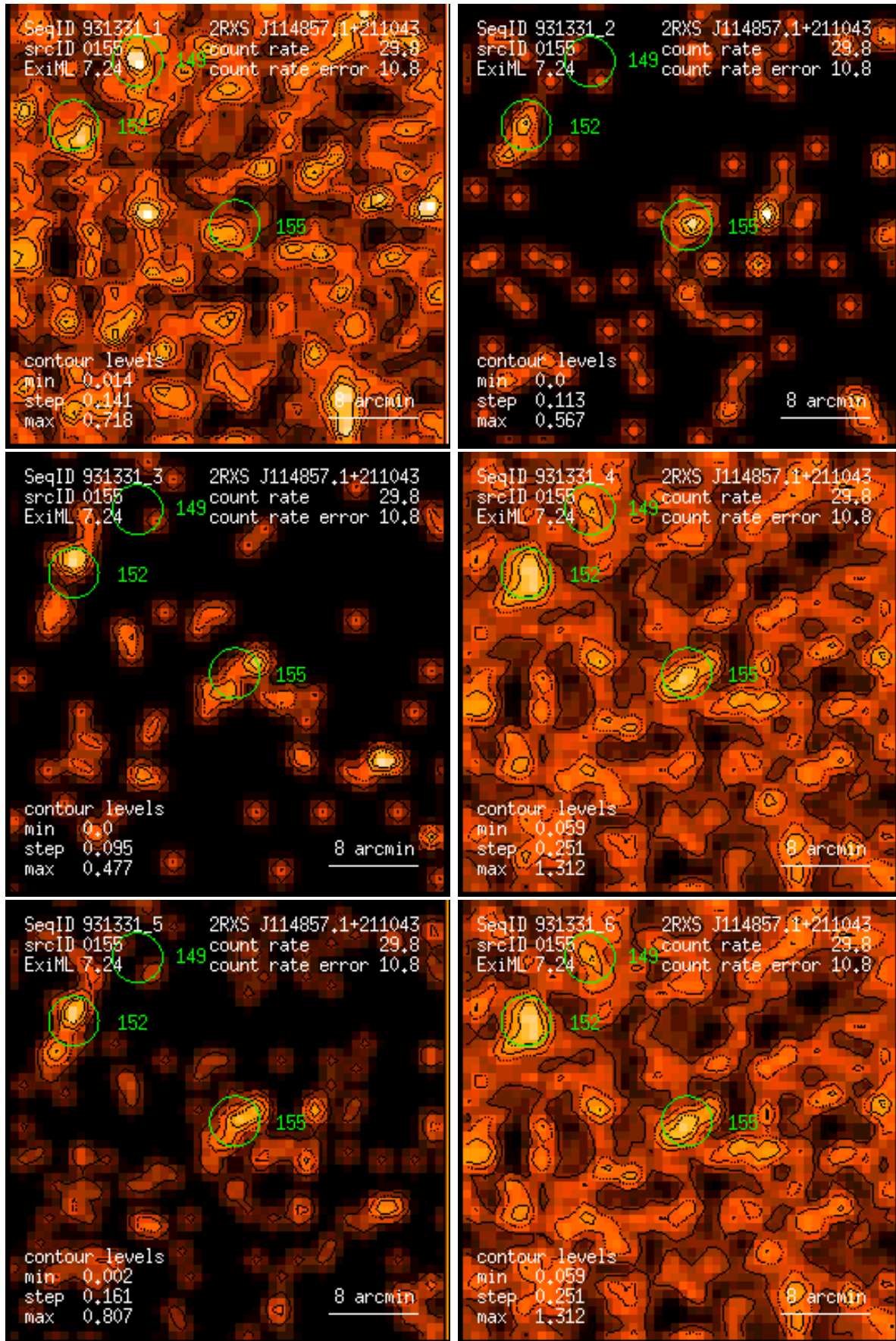
Figure 155: RASS 931331: detection 0155: band rate images, Gaussian filter: (1) PSPC channels 11 – 41, (2) 52 – 90, (3) 91 – 201, (4) 11 – 235, (5) 52 – 201, (6) 11 – 201. Broad band rates in counts/ks. Band rate contour levels in counts/ks/arcmin 2 .
