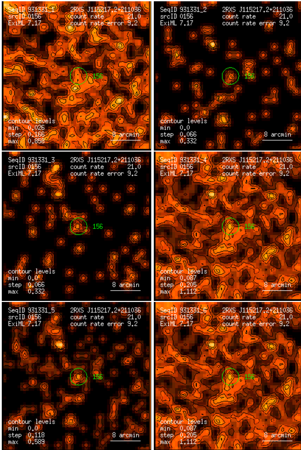
Figure 156: RASS 931331: detection 0156: band rate images, Gaussian filter: (1) PSPC channels 11 – 41, (2) 52 – 90, (3) 91 – 201, (4) 11 – 235, (5) 52 – 201, (6) 11 – 201. Broad band rates in counts/ks. Band rate contour levels in counts/ks/arcmin 2 .
