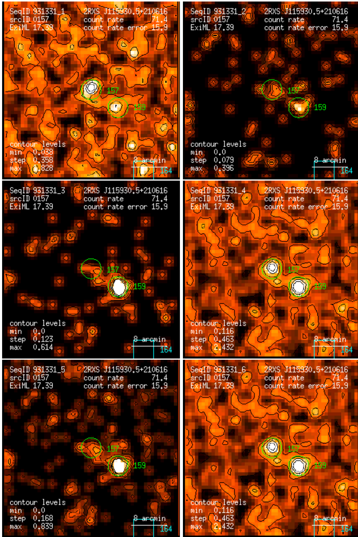
Figure 157: RASS 931331: detection 0157: band rate images, Gaussian filter: (1) PSPC channels 11 – 41, (2) 52 – 90, (3) 91 – 201, (4) 11 – 235, (5) 52 – 201, (6) 11 – 201. Broad band rates in counts/ks. Band rate contour levels in counts/ks/arcmin 2 .
