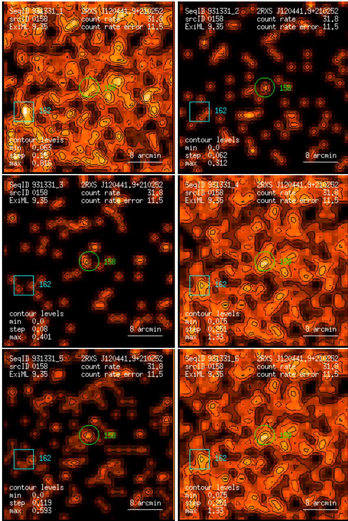
Figure 158: RASS 931331: detection 0158: band rate images, Gaussian filter: (1) PSPC channels 11 – 41, (2) 52 – 90, (3) 91 – 201, (4) 11 – 235, (5) 52 – 201, (6) 11 – 201. Broad band rates in counts/ks. Band rate contour levels in counts/ks/arcmin 2 .
