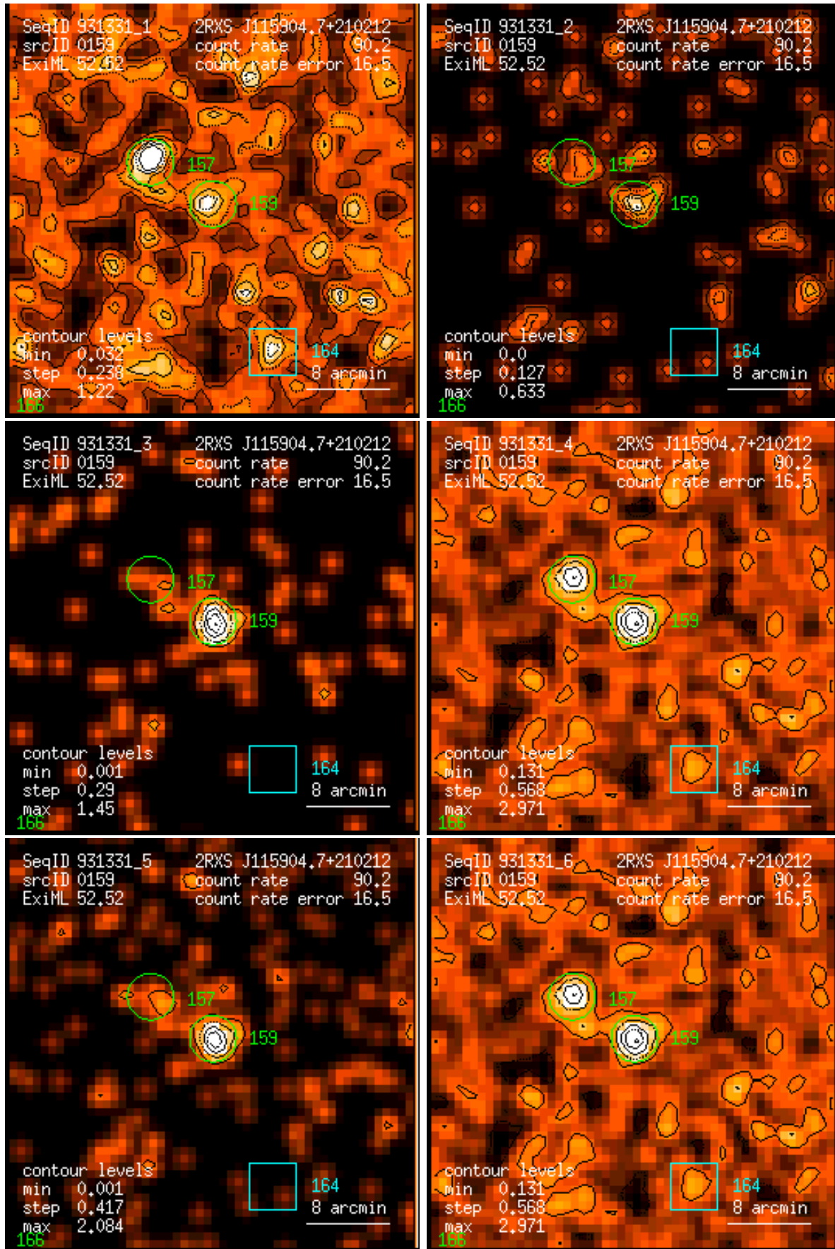
Figure 159: RASS 931331: detection 0159: band rate images, Gaussian filter: (1) PSPC channels 11 – 41, (2) 52 – 90, (3) 91 – 201, (4) 11 – 235, (5) 52 – 201, (6) 11 – 201. Broad band rates in counts/ks. Band rate contour levels in counts/ks/arcmin 2 .
