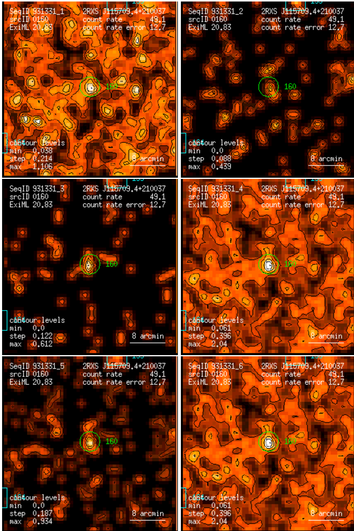
Figure 160: RASS 931331: detection 0160: band rate images, Gaussian filter: (1) PSPC channels 11 – 41, (2) 52 – 90, (3) 91 – 201, (4) 11 – 235, (5) 52 – 201, (6) 11 – 201. Broad band rates in counts/ks. Band rate contour levels in counts/ks/arcmin 2 .
