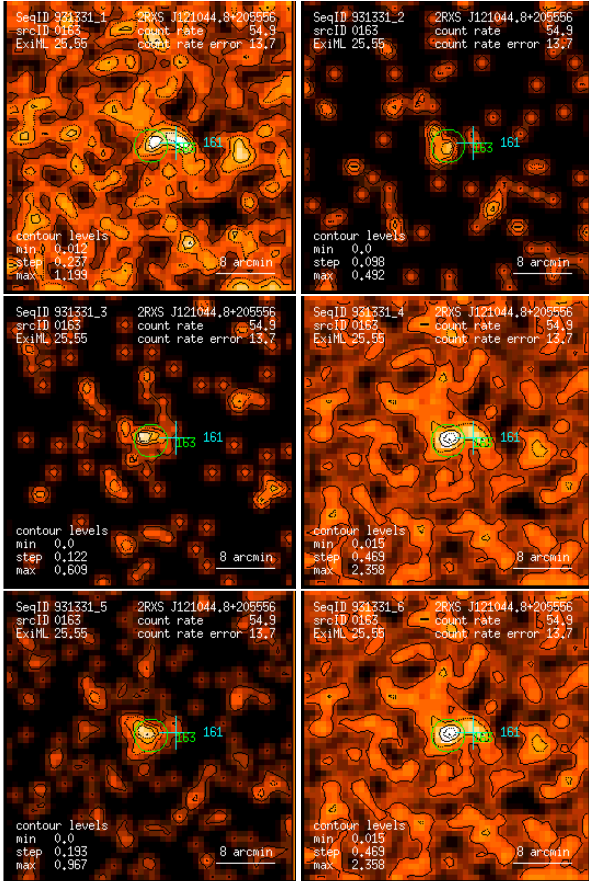
Figure 163: RASS 931331: detection 0163: band rate images, Gaussian filter: (1) PSPC channels 11 – 41, (2) 52 – 90, (3) 91 – 201, (4) 11 – 235, (5) 52 – 201, (6) 11 – 201. Broad band rates in counts/ks. Band rate contour levels in counts/ks/arcmin 2 .
