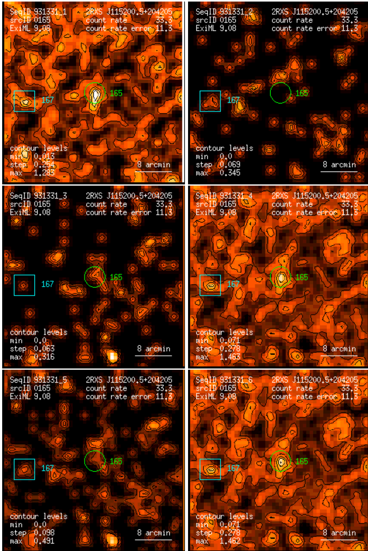
Figure 165: RASS 931331: detection 0165: band rate images, Gaussian filter: (1) PSPC channels 11 – 41, (2) 52 – 90, (3) 91 – 201, (4) 11 – 235, (5) 52 – 201, (6) 11 – 201. Broad band rates in counts/ks. Band rate contour levels in counts/ks/arcmin 2 .
