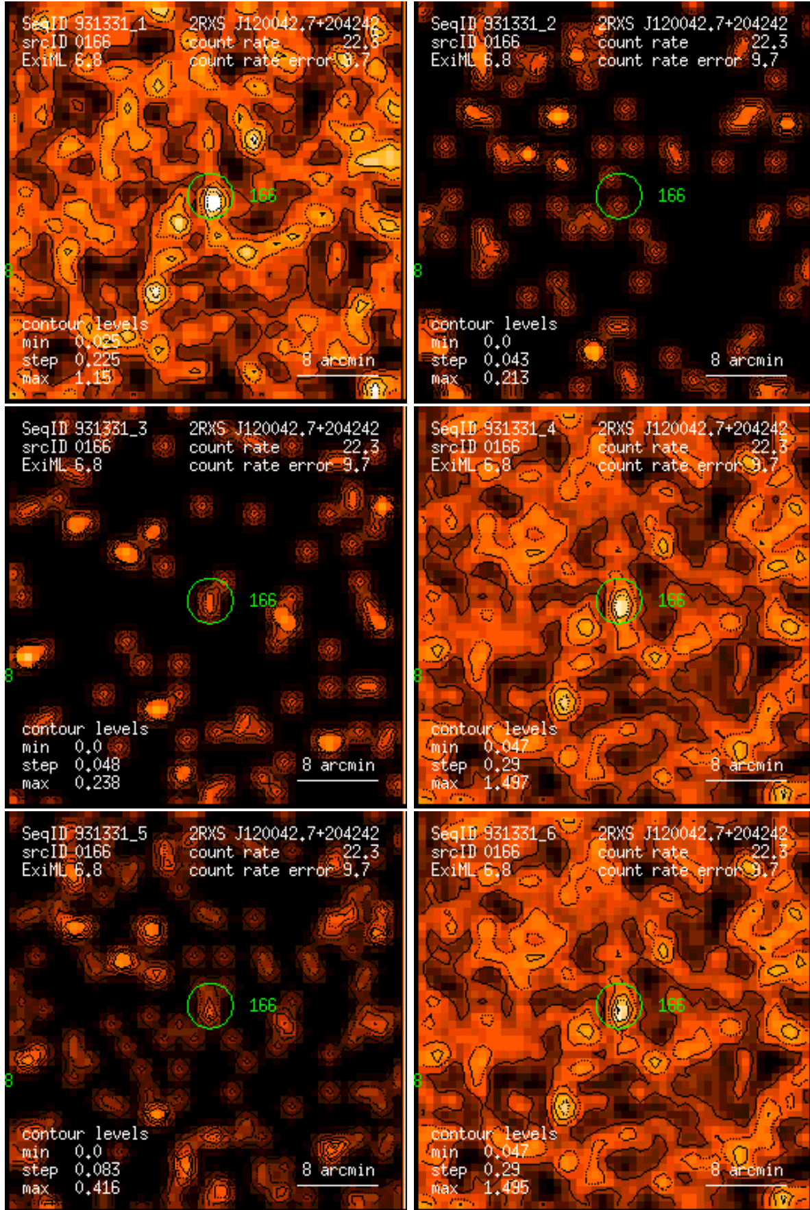
Figure 166: RASS 931331: detection 0166: band rate images, Gaussian filter: (1) PSPC channels 11 – 41, (2) 52 – 90, (3) 91 – 201, (4) 11 – 235, (5) 52 – 201, (6) 11 – 201. Broad band rates in counts/ks. Band rate contour levels in counts/ks/arcmin 2 .
